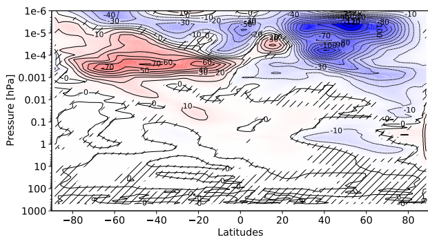
(e) \Delta \nabla \cdot \mathbf{F}
