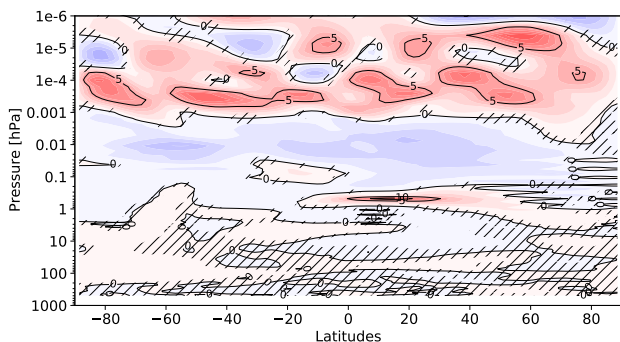
(c) \Delta \vec{v}^*
