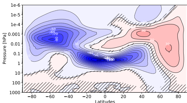
(b) \Delta z zonal wind
