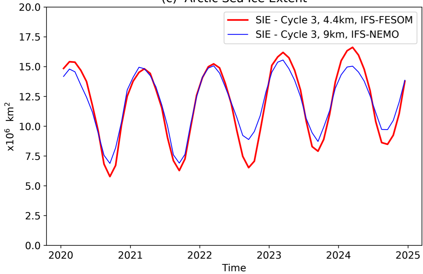
(c) Arctic Sea Ice Extent
