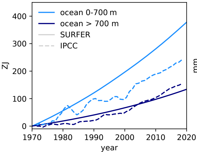
Energy change in ocean 1971-2018
