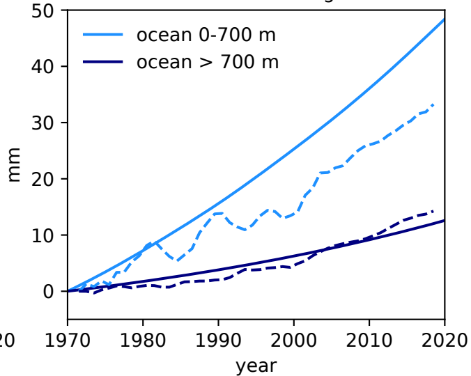
Thermosteric Sea level change 1971-2018
