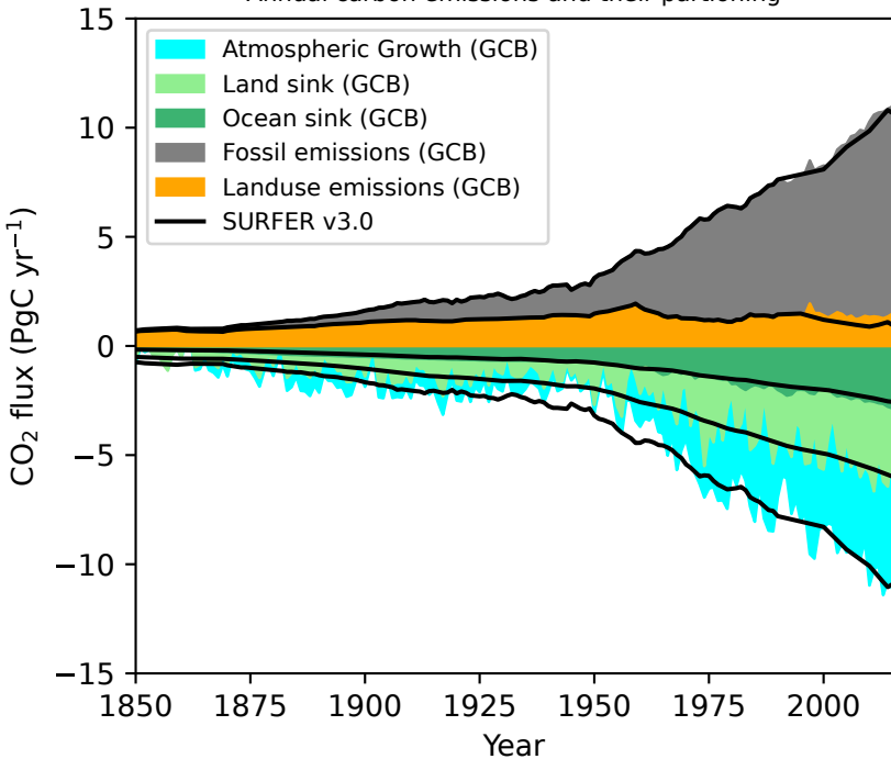
Annual carbon emissions and their partitioning
