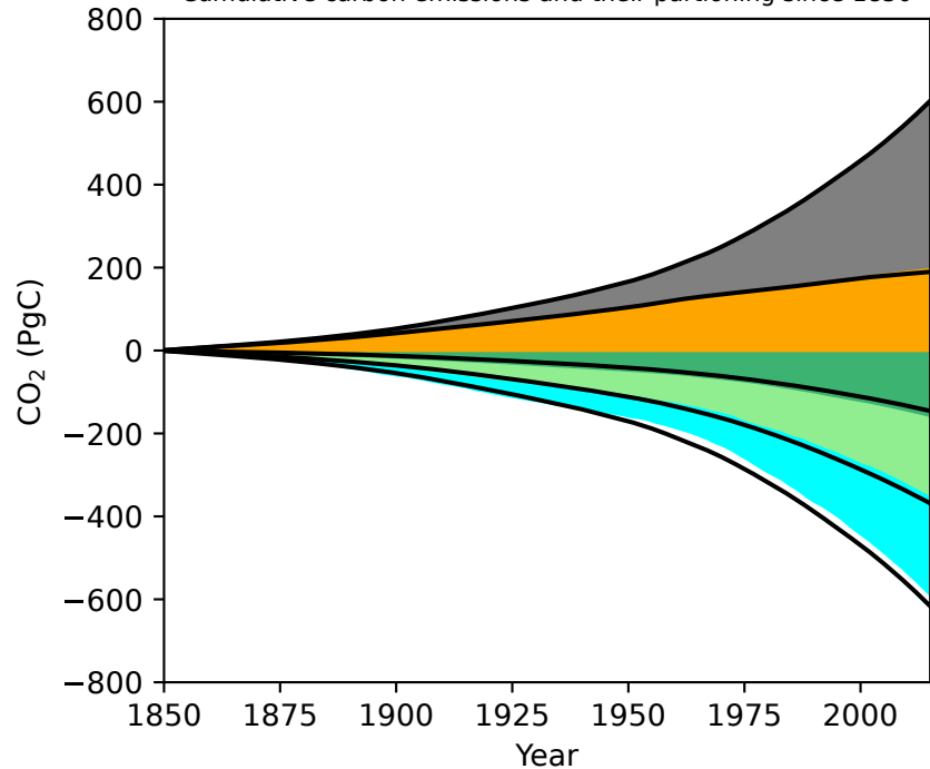
Cumulative carbon emissions and their partitioning since 1850
