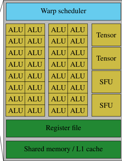
Streaming multiprocessor
