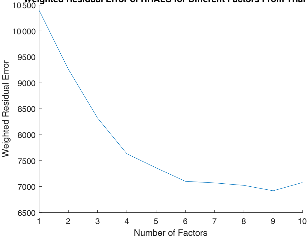
Weighted Residual Error of RHALS for Different Factors From Trial 13
