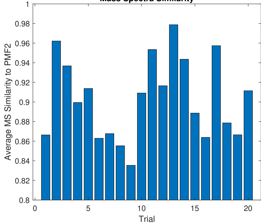
Mass Spectra Similarity
