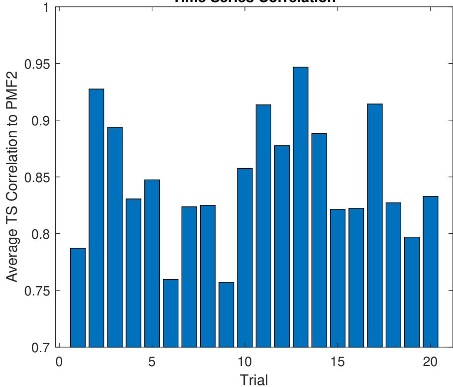
Time Series Correlation
