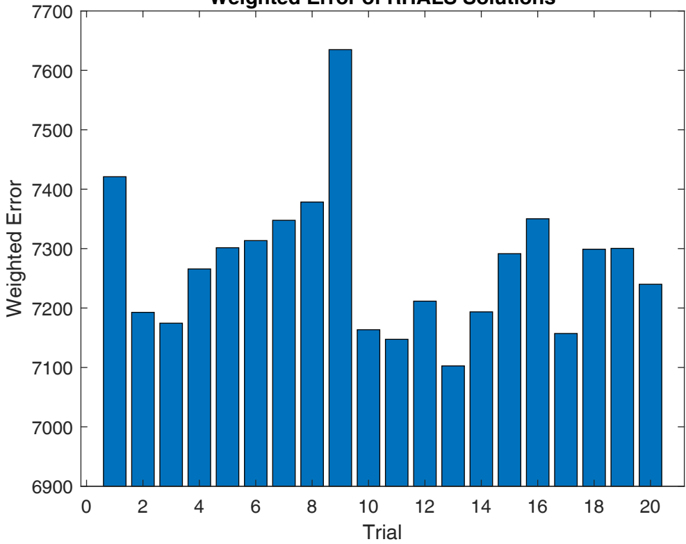
Weighted Error of RHALS Solutions
