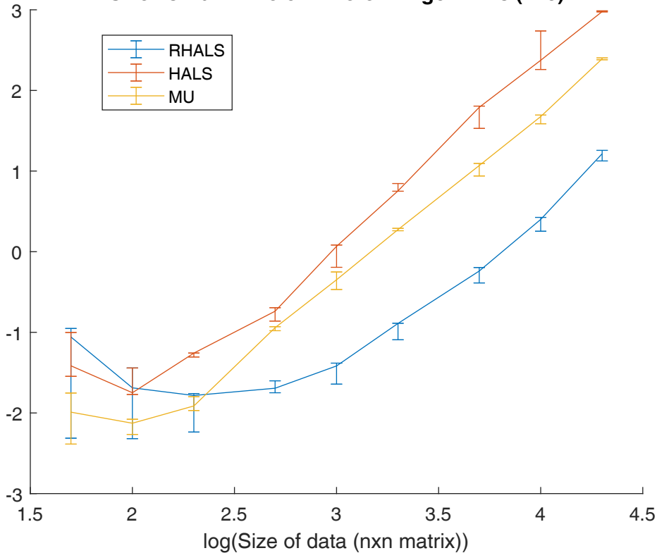
Size vs Run Time of Different Algorithms (k=5)
