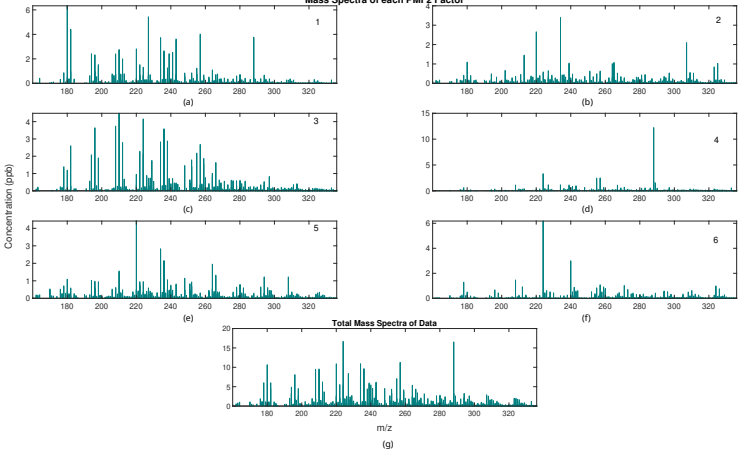
Mass Spectra of each PMF2 Factor
