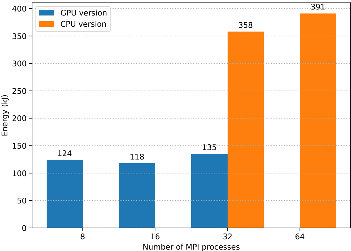
Adastra: Energy consumption on 1 node (FFT)
