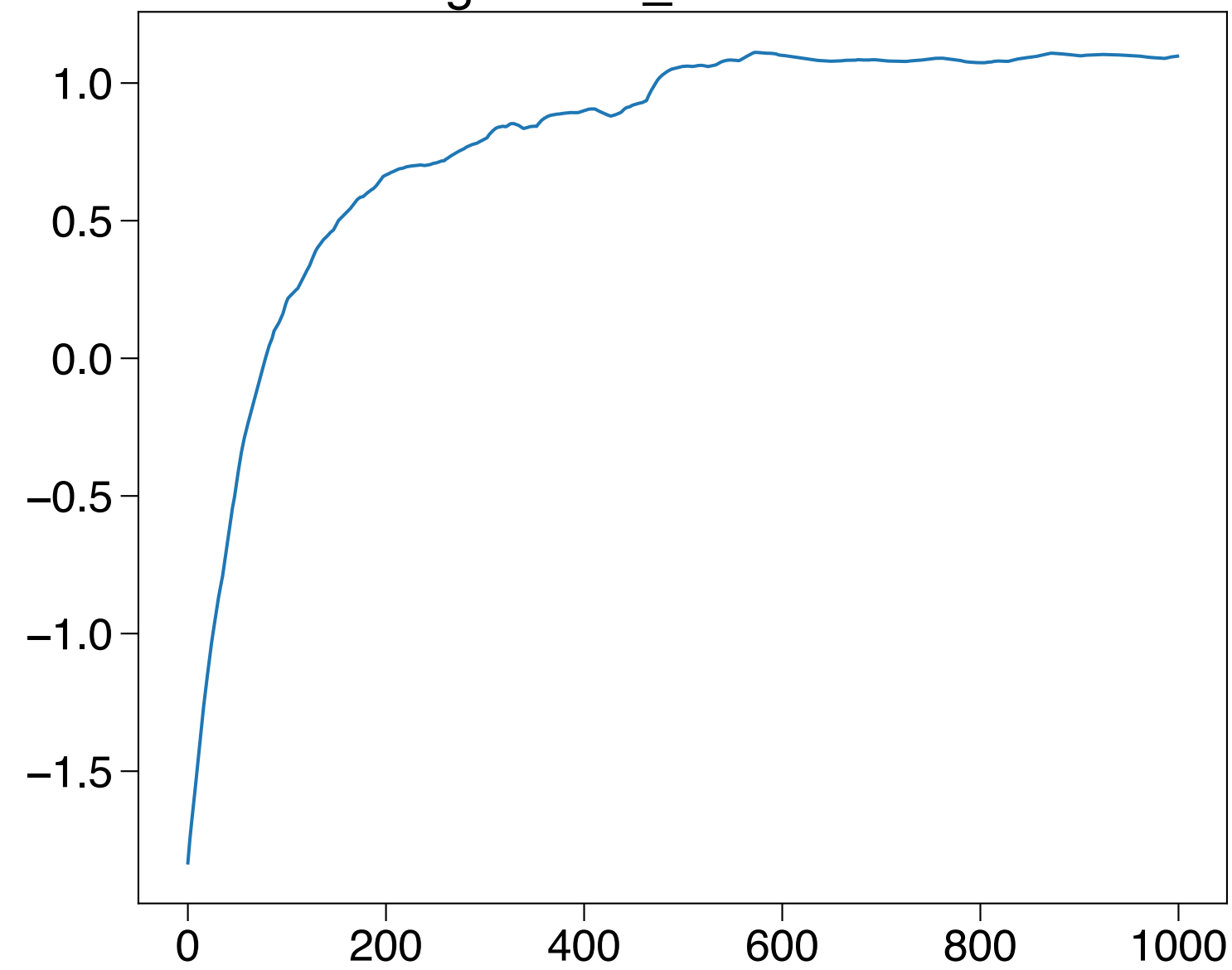
lengthscale_loc: 1.097748
