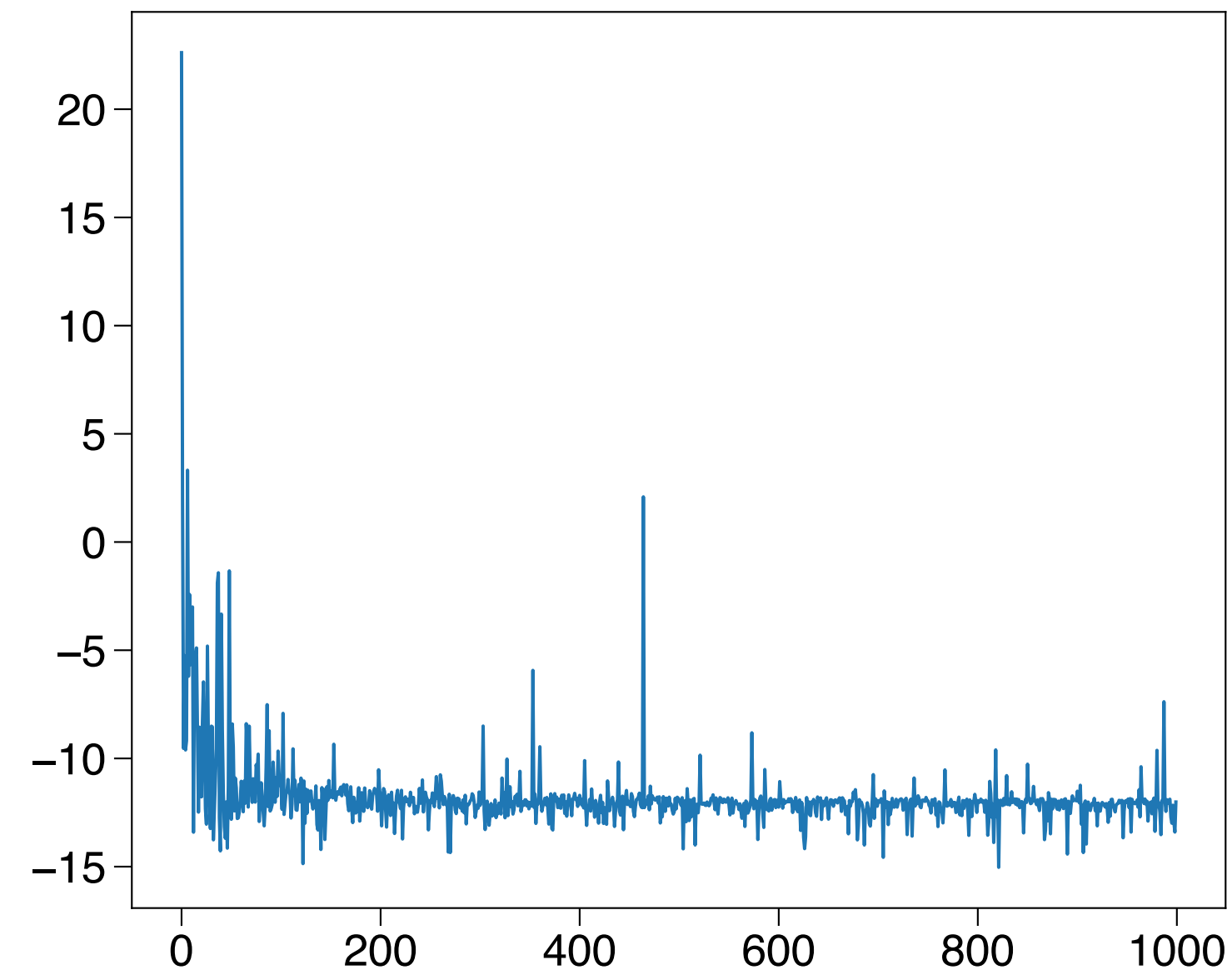
loss: -12.013354
