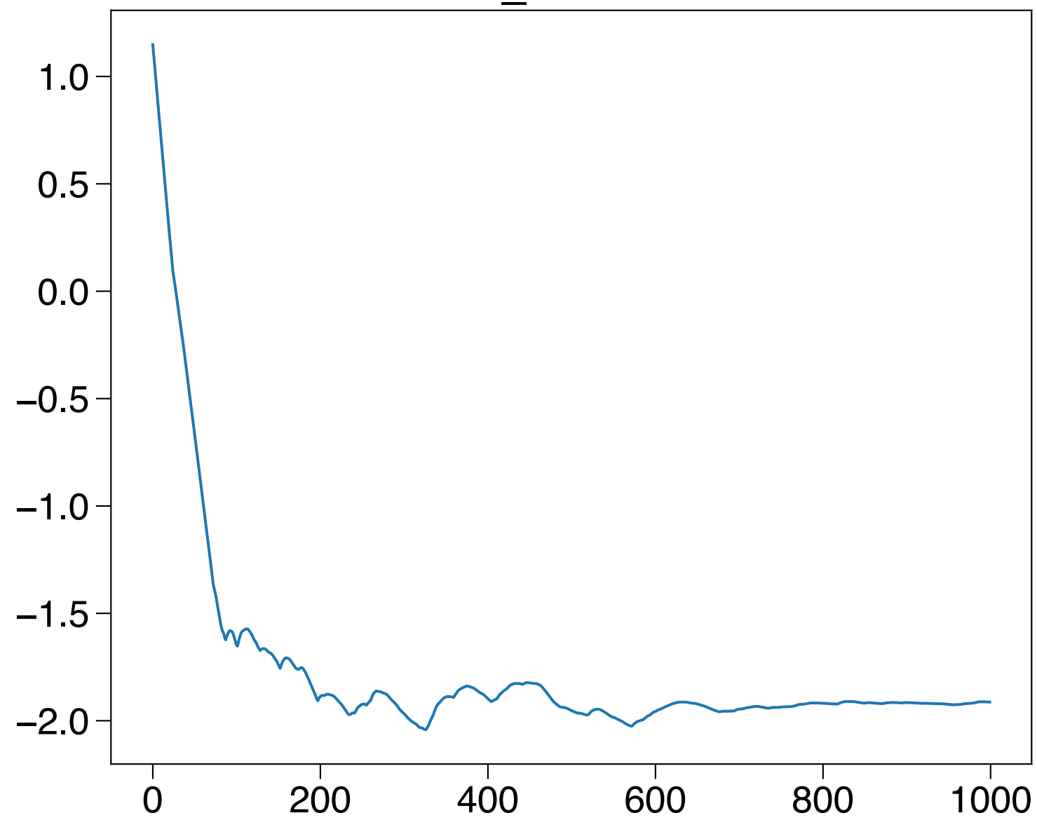
variance_loc: -1.913146
