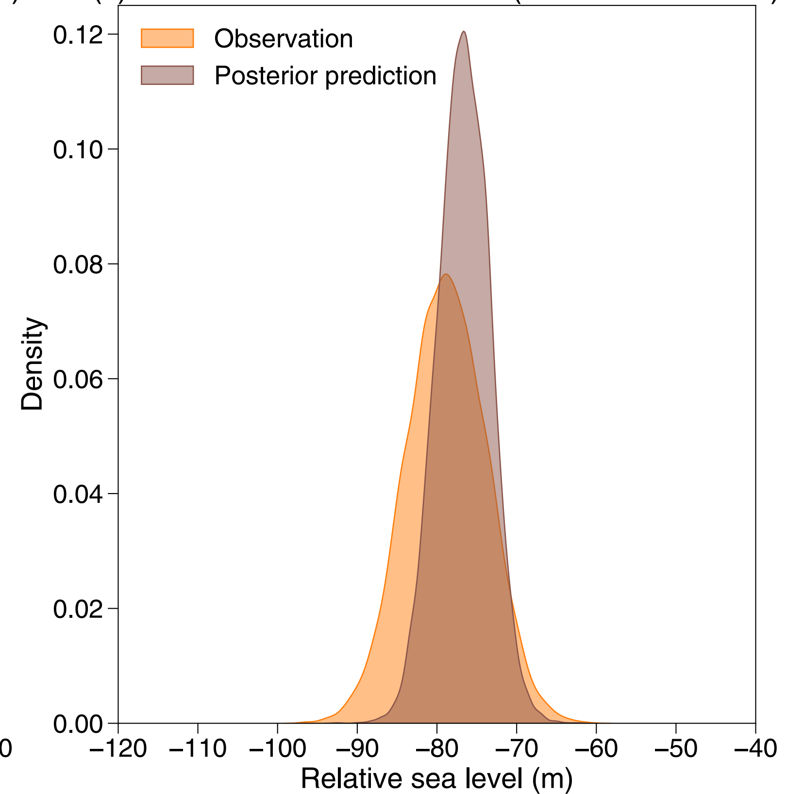
(c) Posterior Predictive Check (Normal Likelihood)
