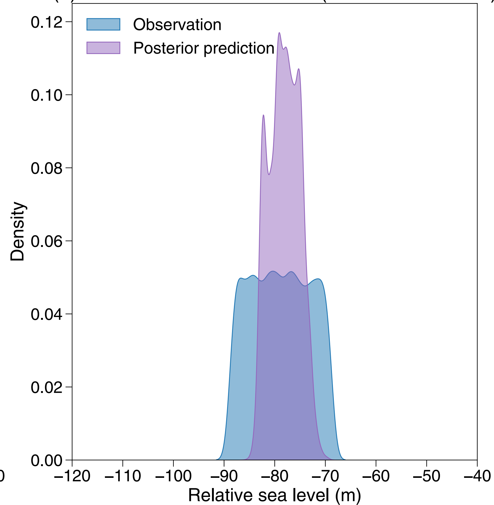
(b) Posterior Predictive Check (Uniform Likelihood)
