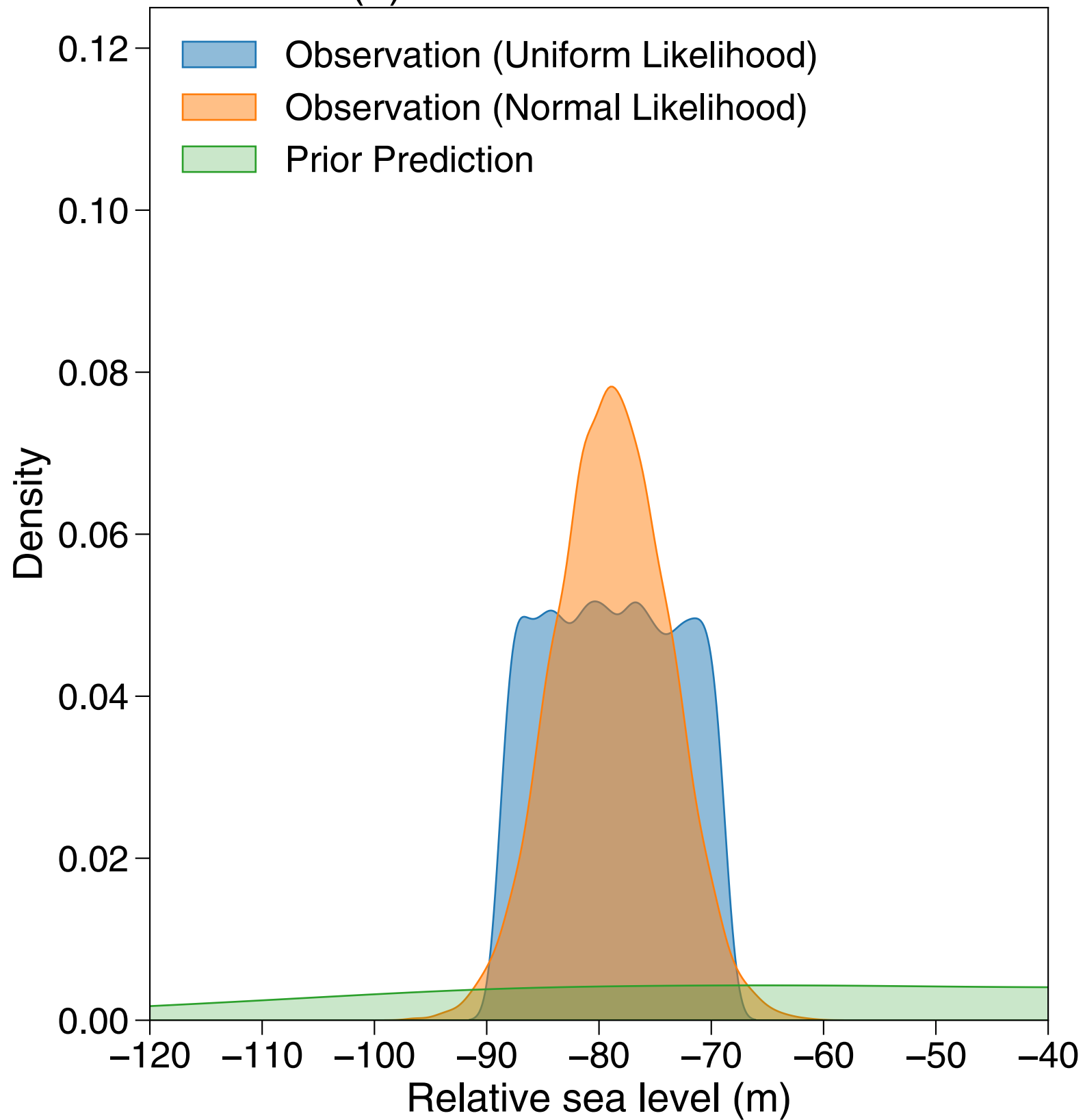
(a) Prior Predictive Check
