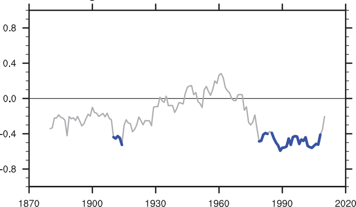
Running corr: JJA0 ATL3 and DJF1 Niño 3.4
