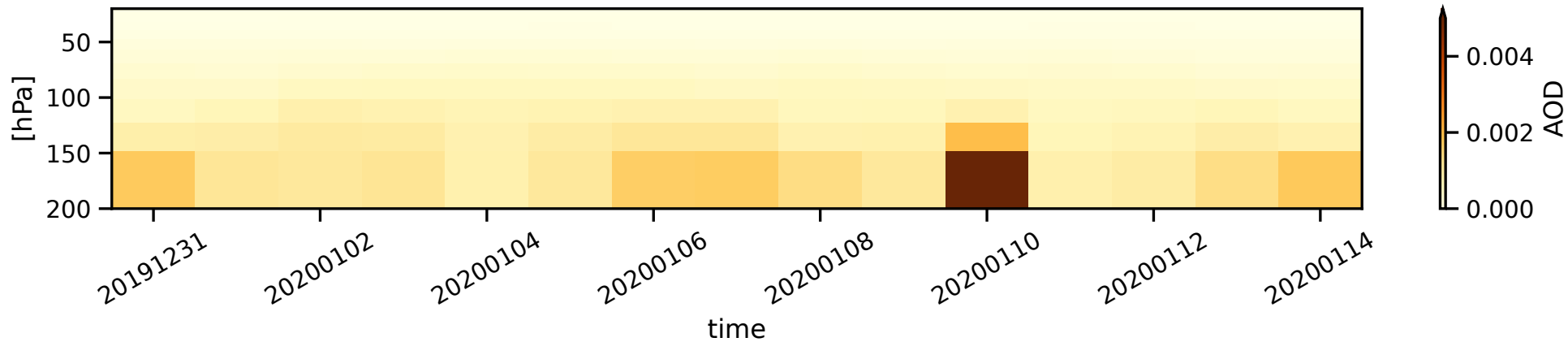
(a) 550nm AOD at 25°-30°S 150°-155°E
