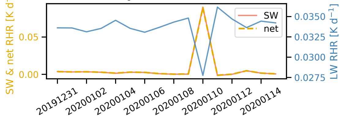
(c) Radiative heating rate at 25°-30°S 150°-155°E
