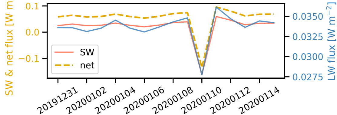
(b) Radiative flux at 25°-30°S 150°-155°E
