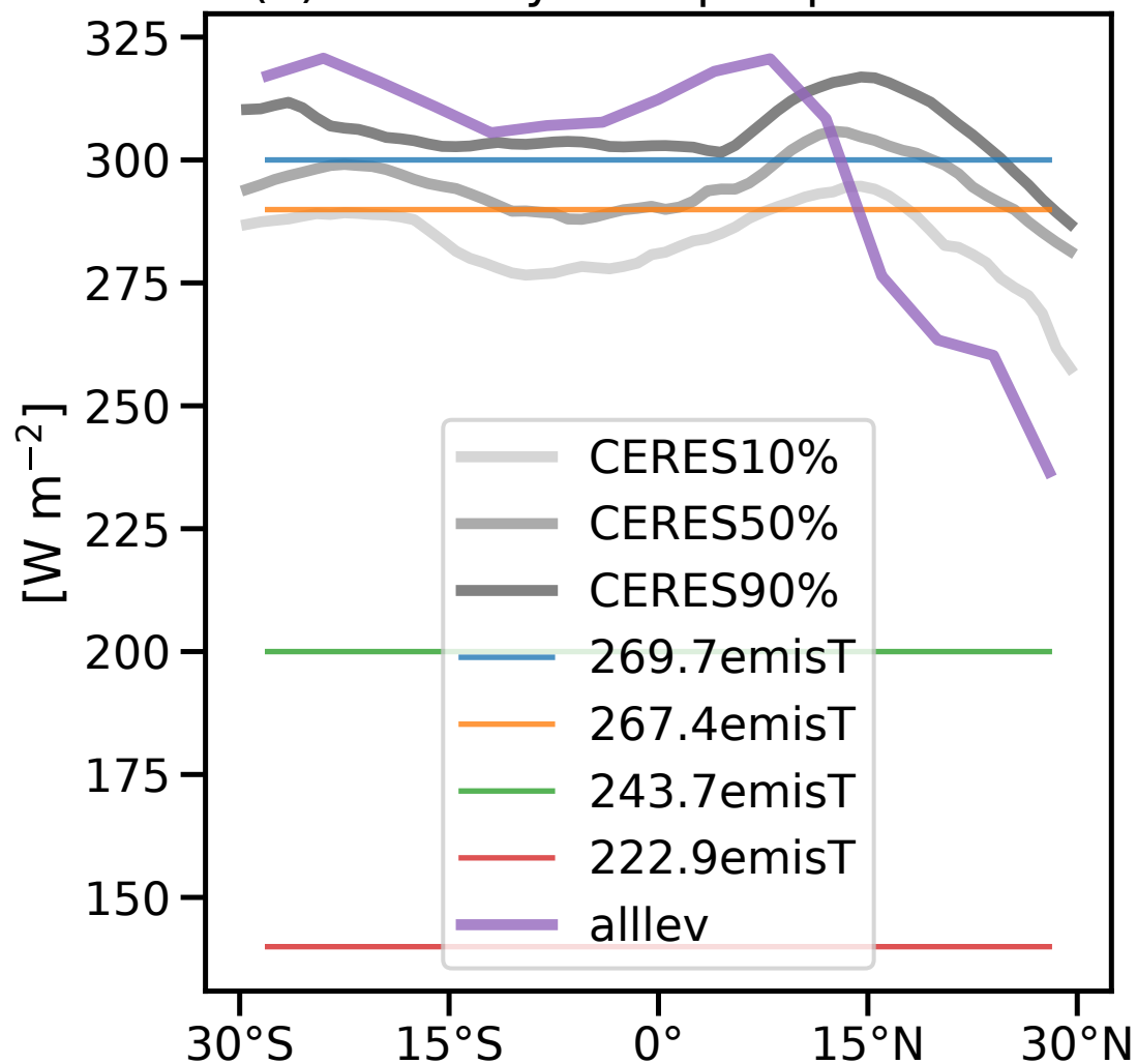
(a) clear-sky 200hpa upward flux
