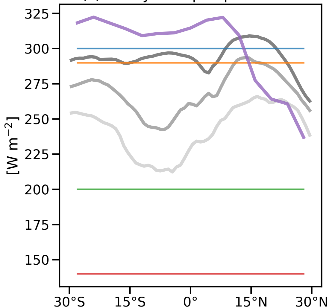
(c) all-sky 200hpa upward flux
