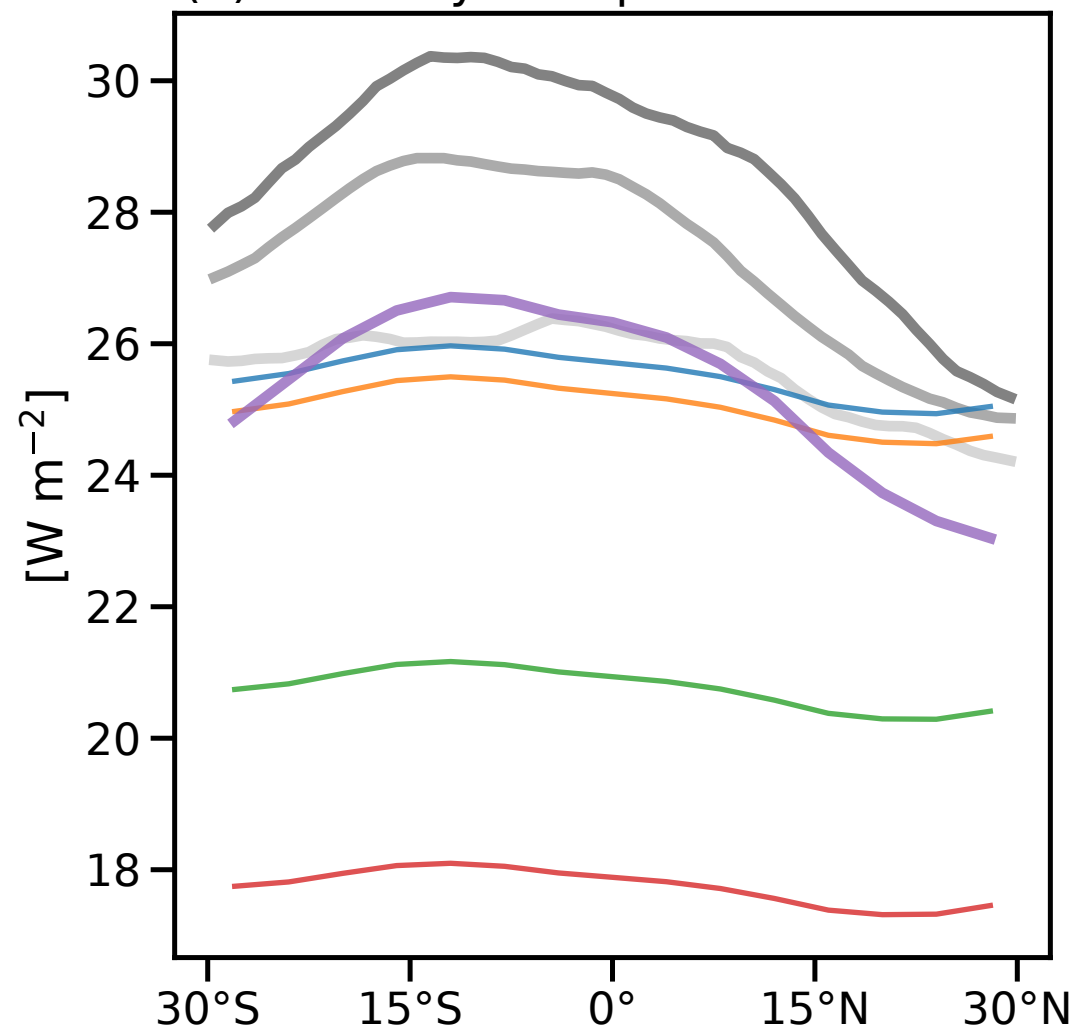
(b) clear-sky 200hpa downward flux
