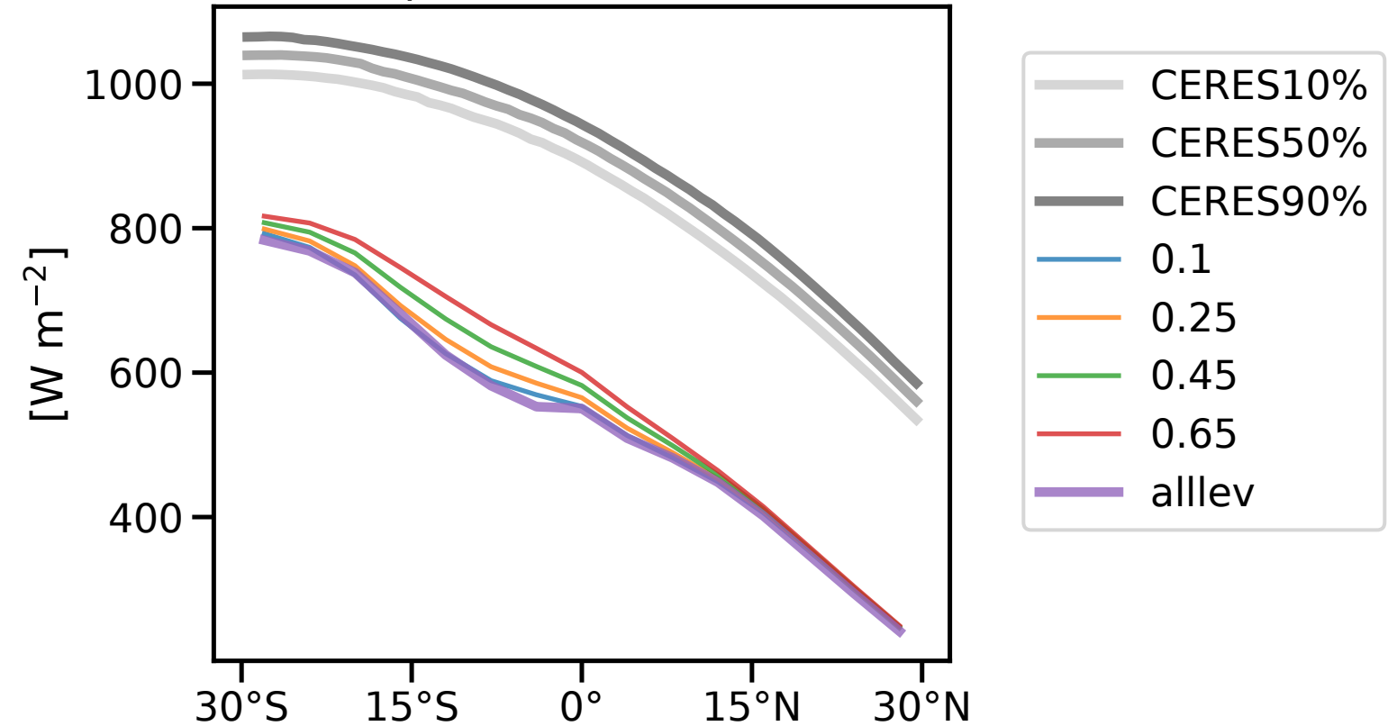
(c) 200hpa downward flux at T15
