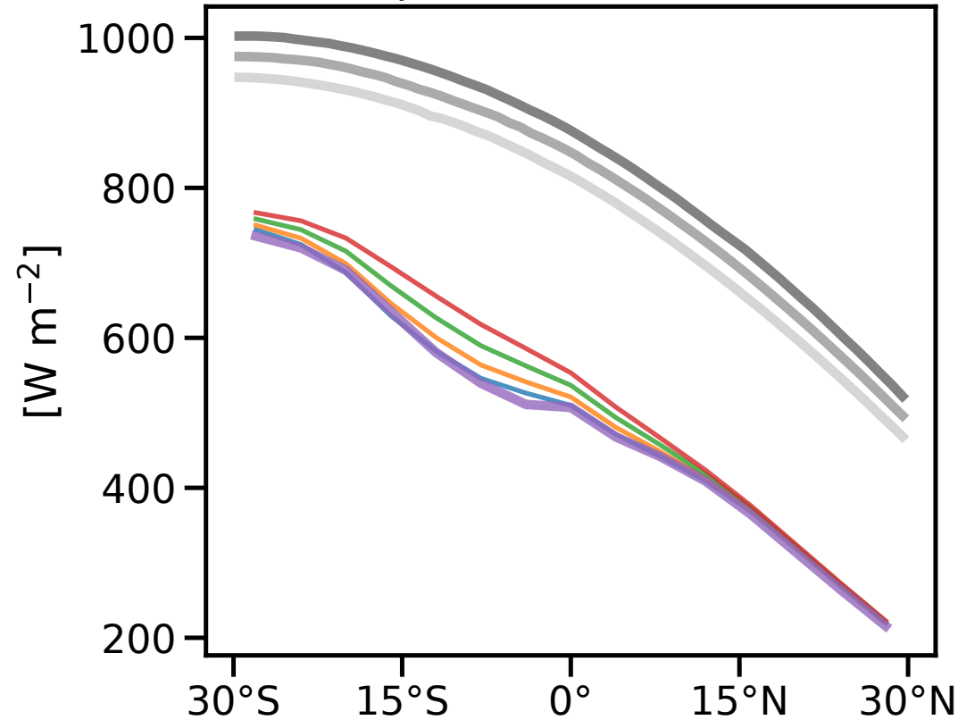
(a) 200hpa downward flux at T09
