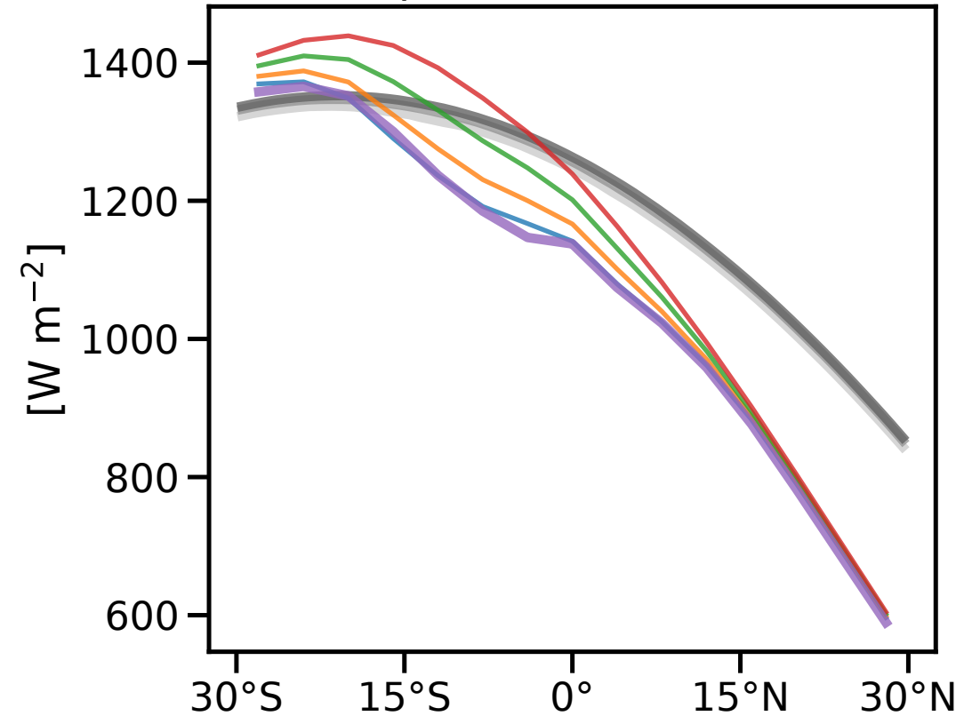
(b) 200hpa downward flux at T12
