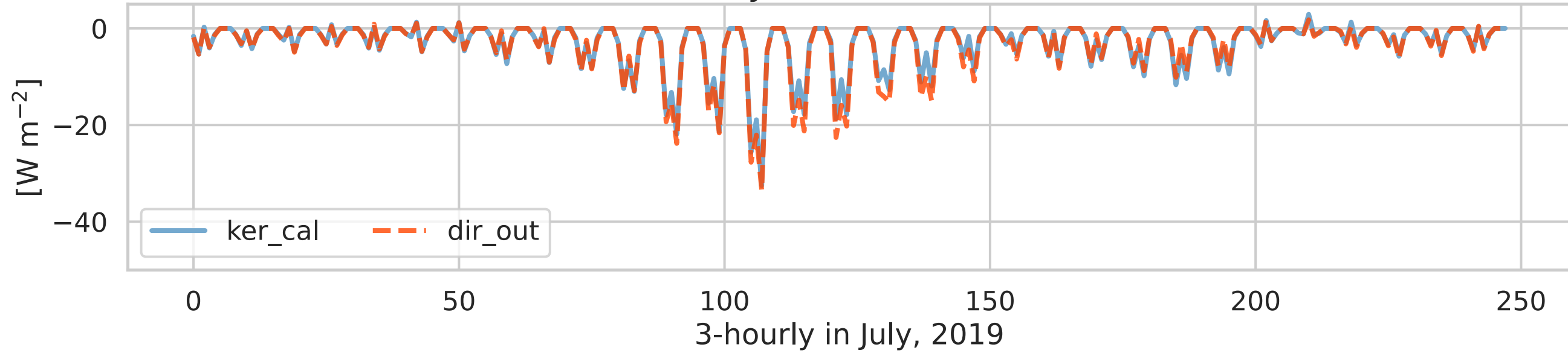
(a) ARE of clr-sky SW TOA flux at 25°N90°E
