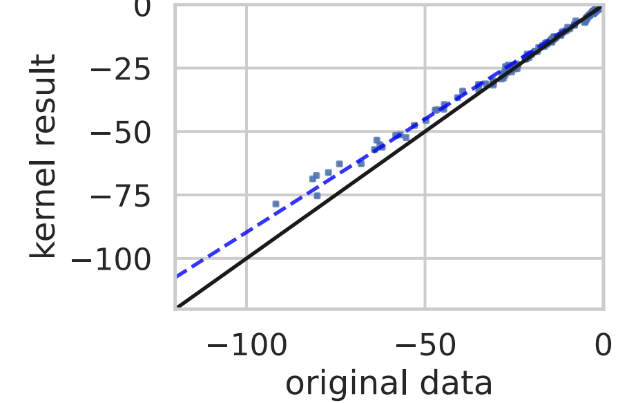
(e) ARE of SW srf flux
