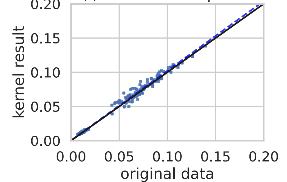
(f) ARE of SW trop RHR
