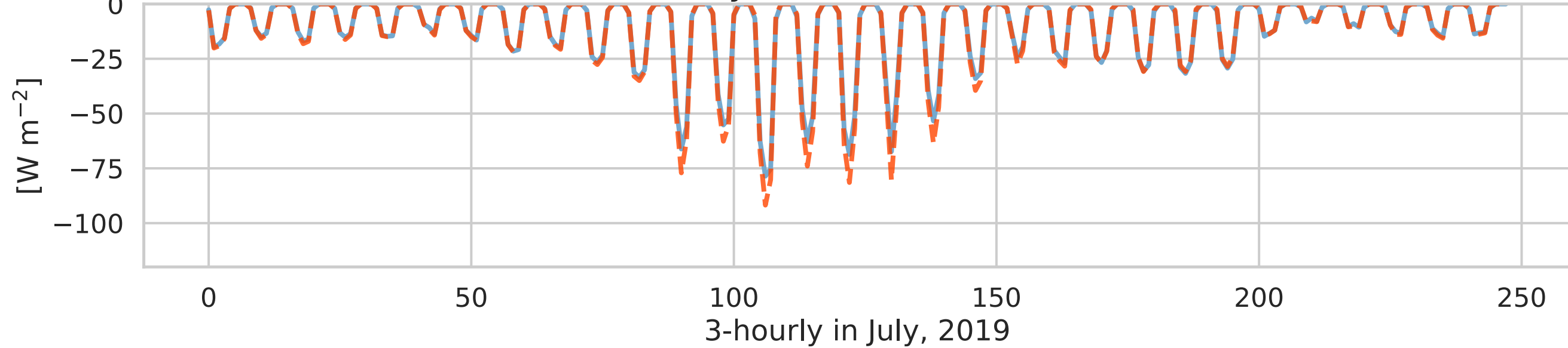
(b) ARE of clr-sky SW surface flux at 25°N90°E
