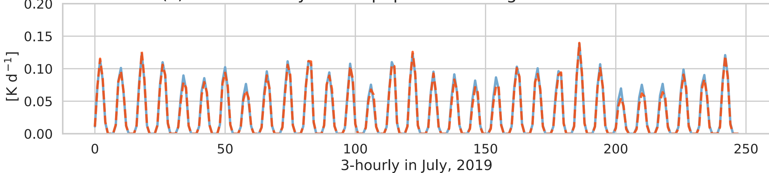
(c) ARE of clr-sky SW tropopause heating rate at 25°N90°E
