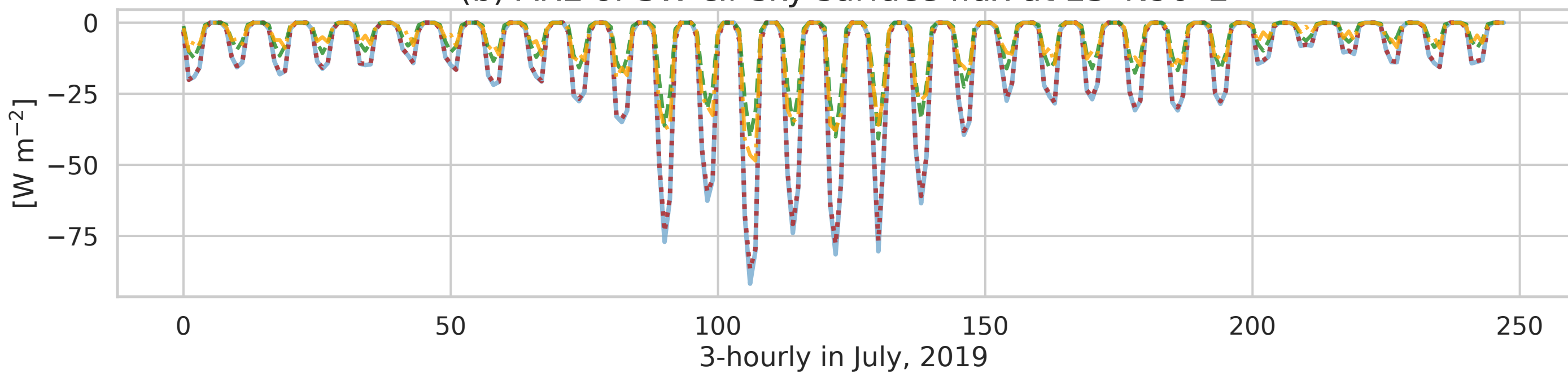
(c) ARE of SW clr-sky tropopause heating rate at 25°N90°E
