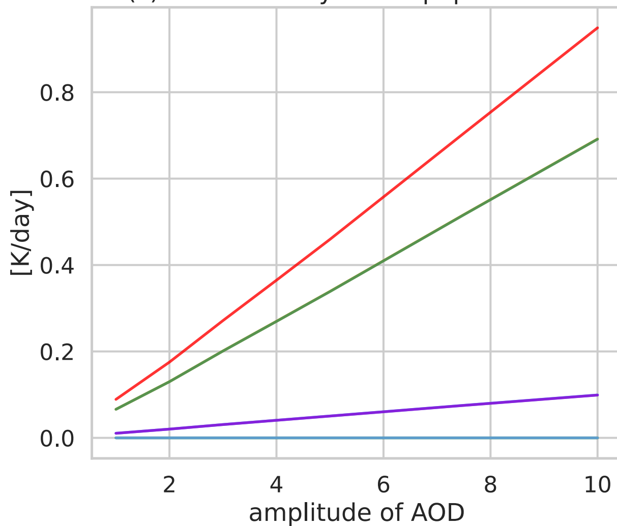
(c) ARE of clr-sky SW tropopause RHR
