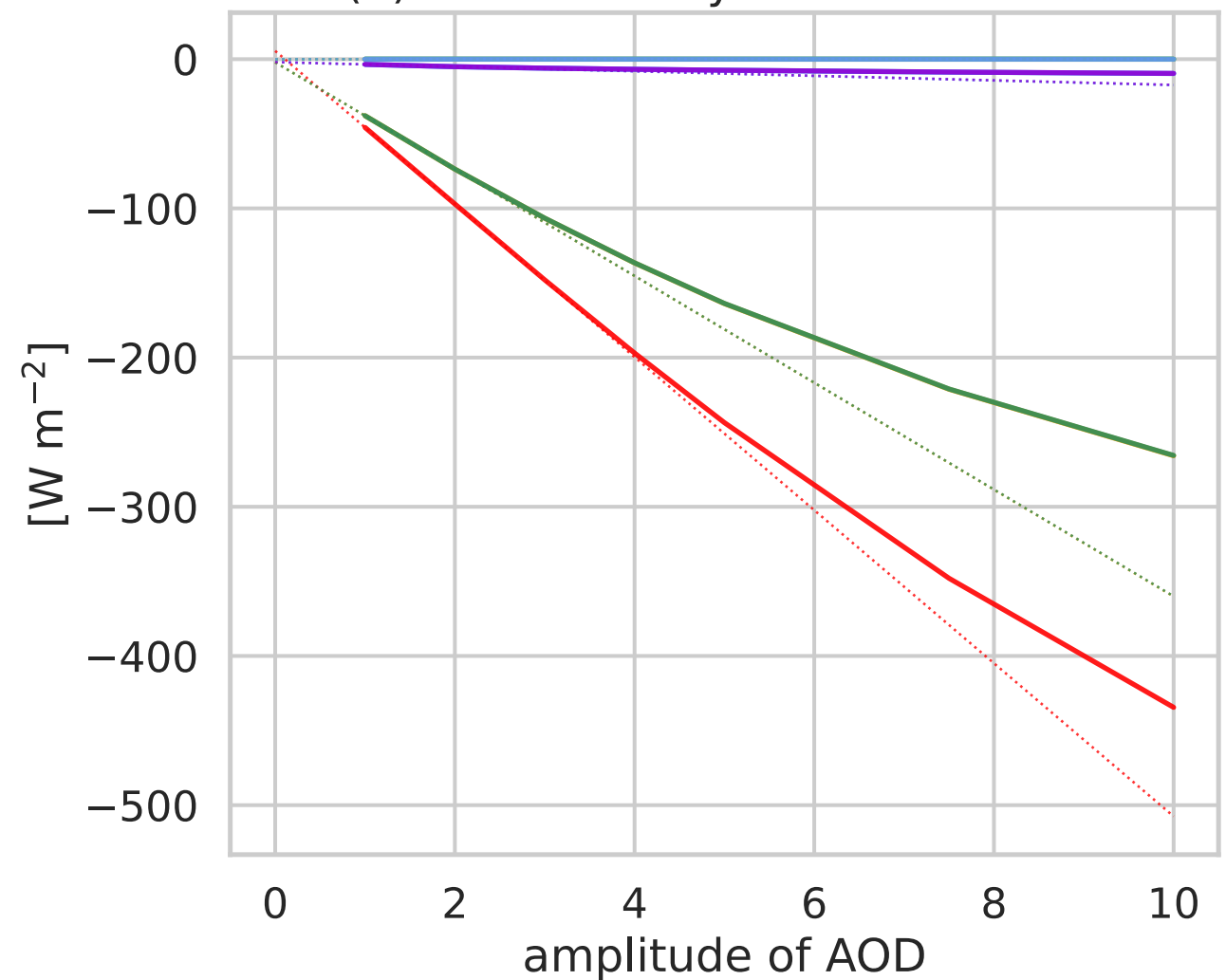
(b) ARE of clr-sky SW surface flux
