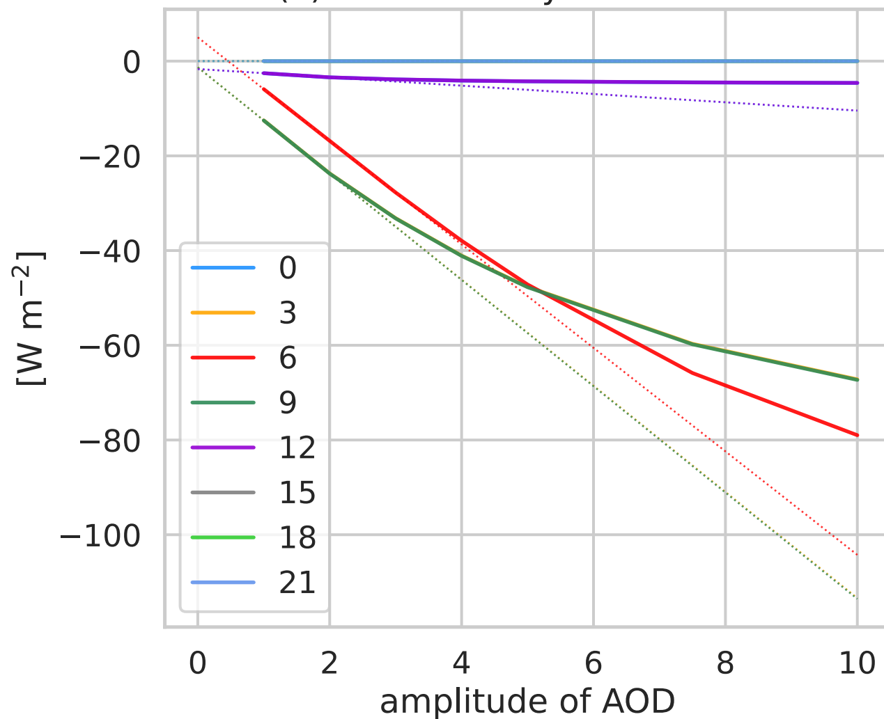
(a) ARE of clr-sky SW TOA flux
