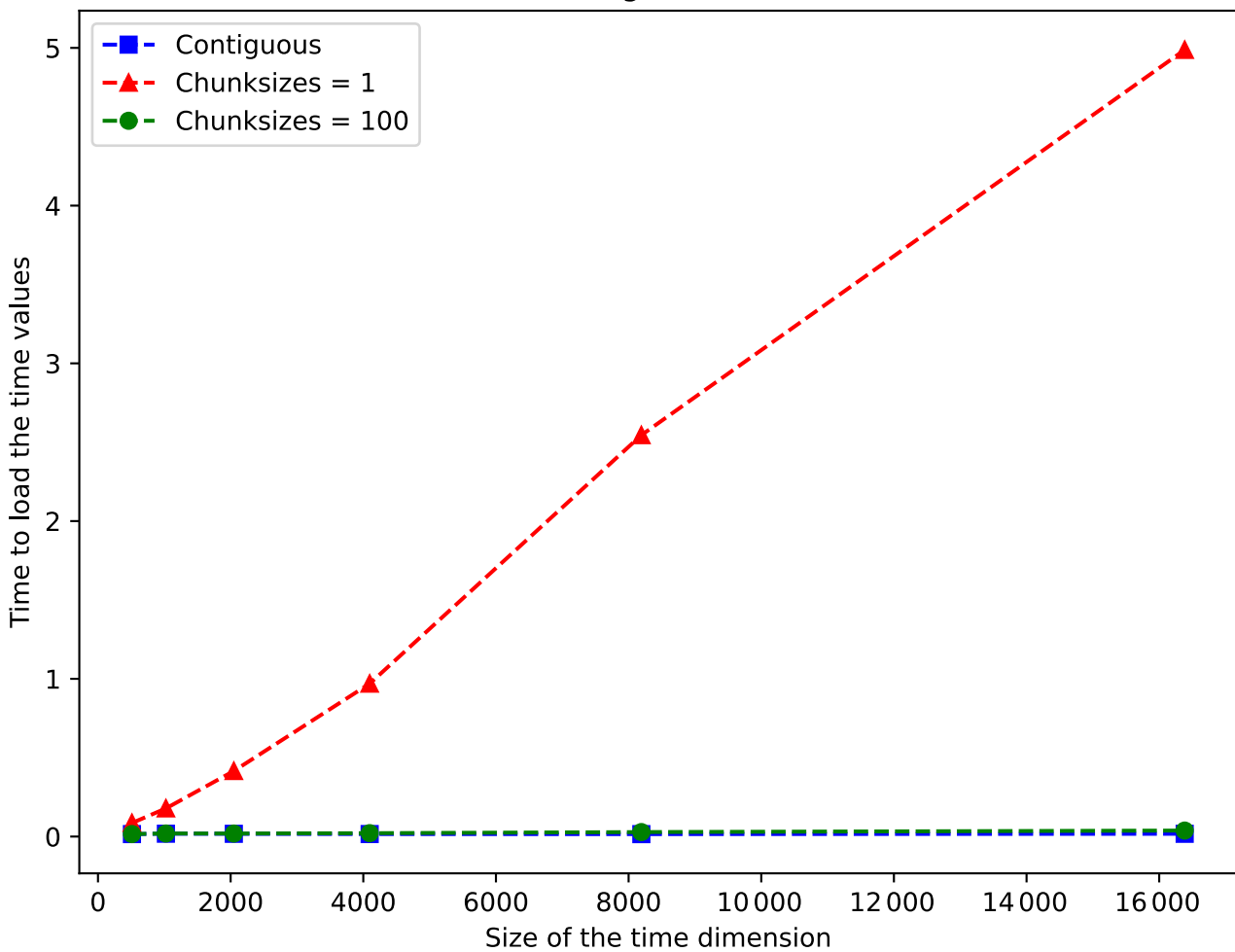
Performance of different chunking schemes for different dataset sizes.
