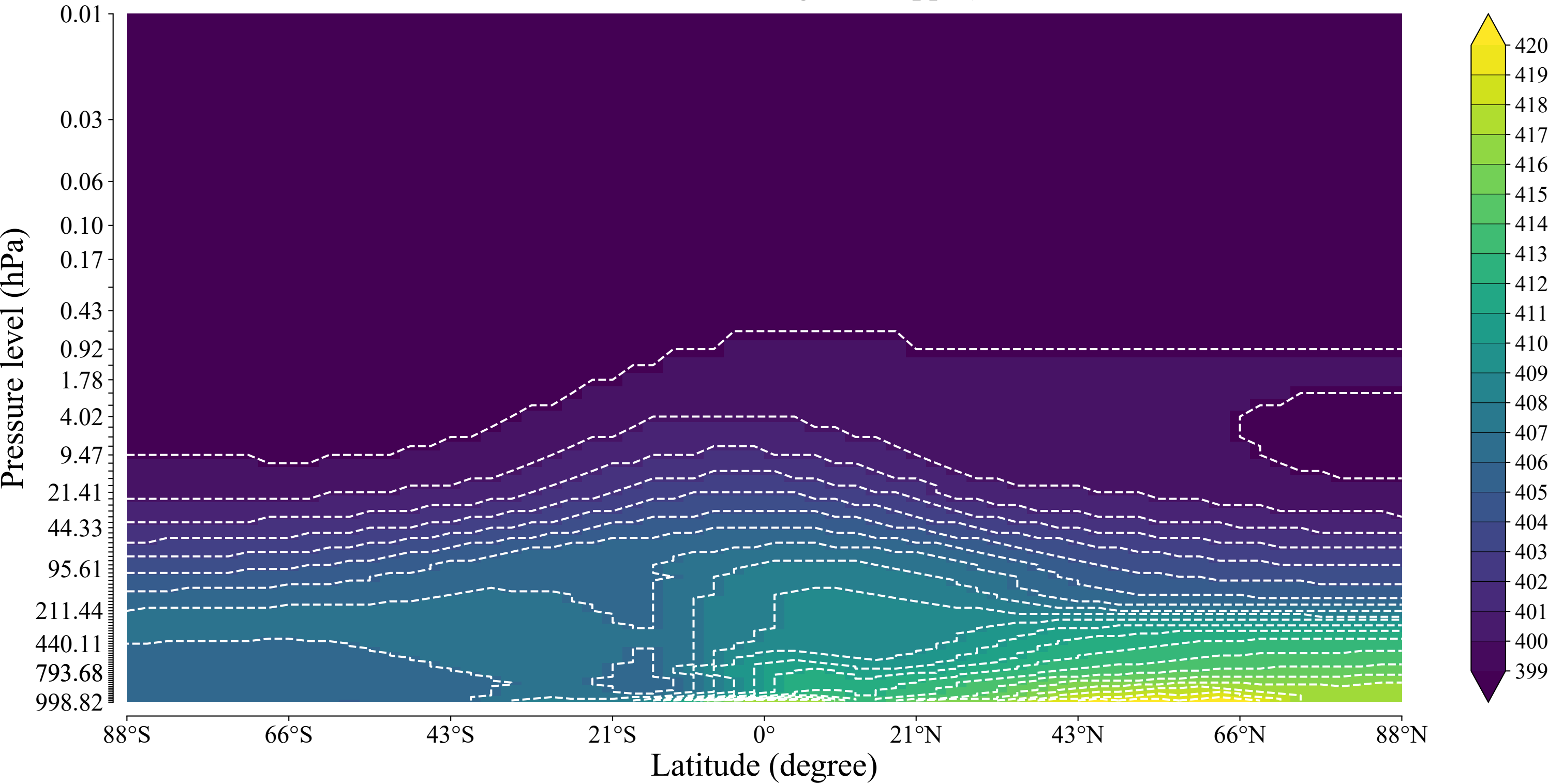
CO 2 volume mixing ratios (ppm)
