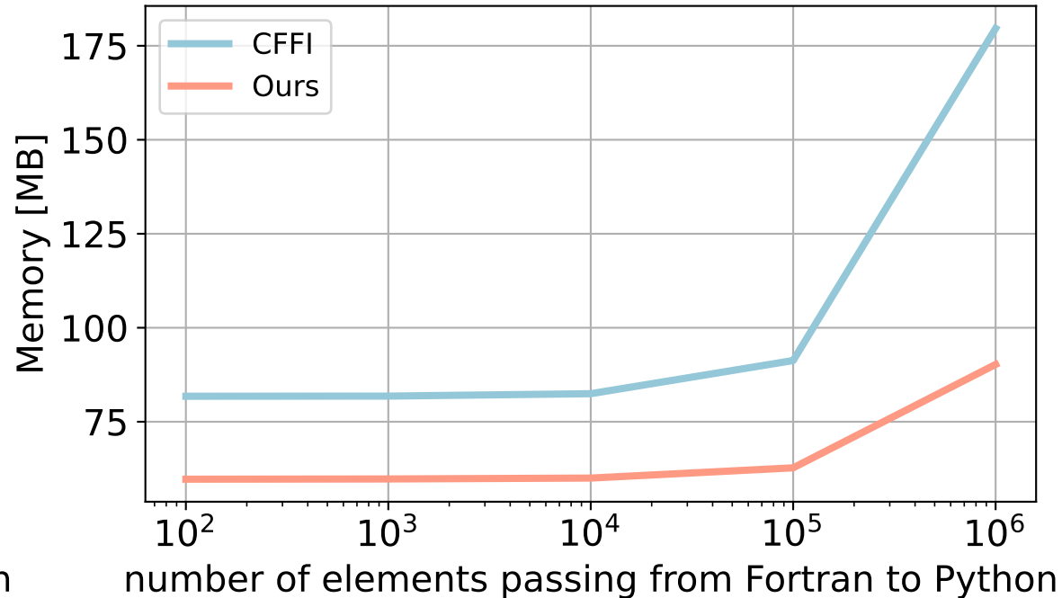
(b) Memory usage
