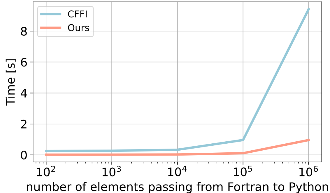
(a) Computational time
