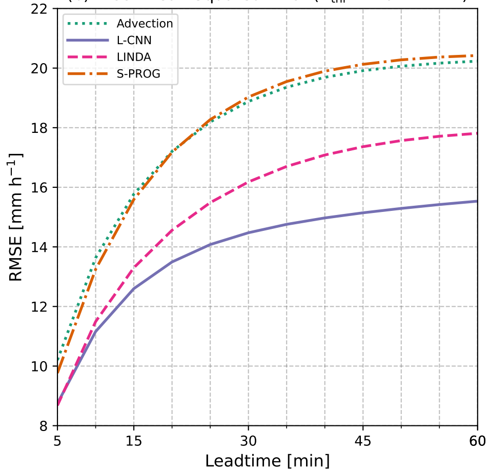
(b) Root Mean Squared Error ( R_{\text{thr}} = 4.6 \text{ mm h}^{-1} )
