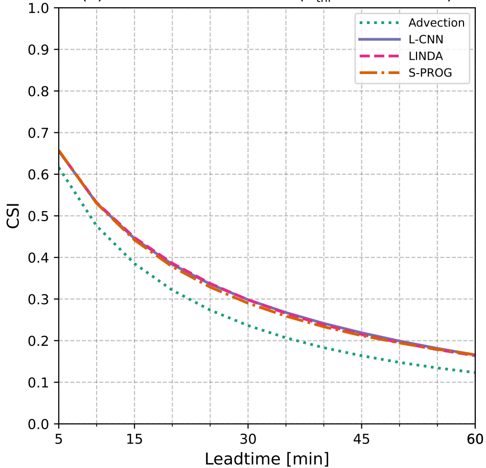
(a) Critical Success Index ( R_{\text{thr}} = 4.6 \text{ mm h}^{-1} )
