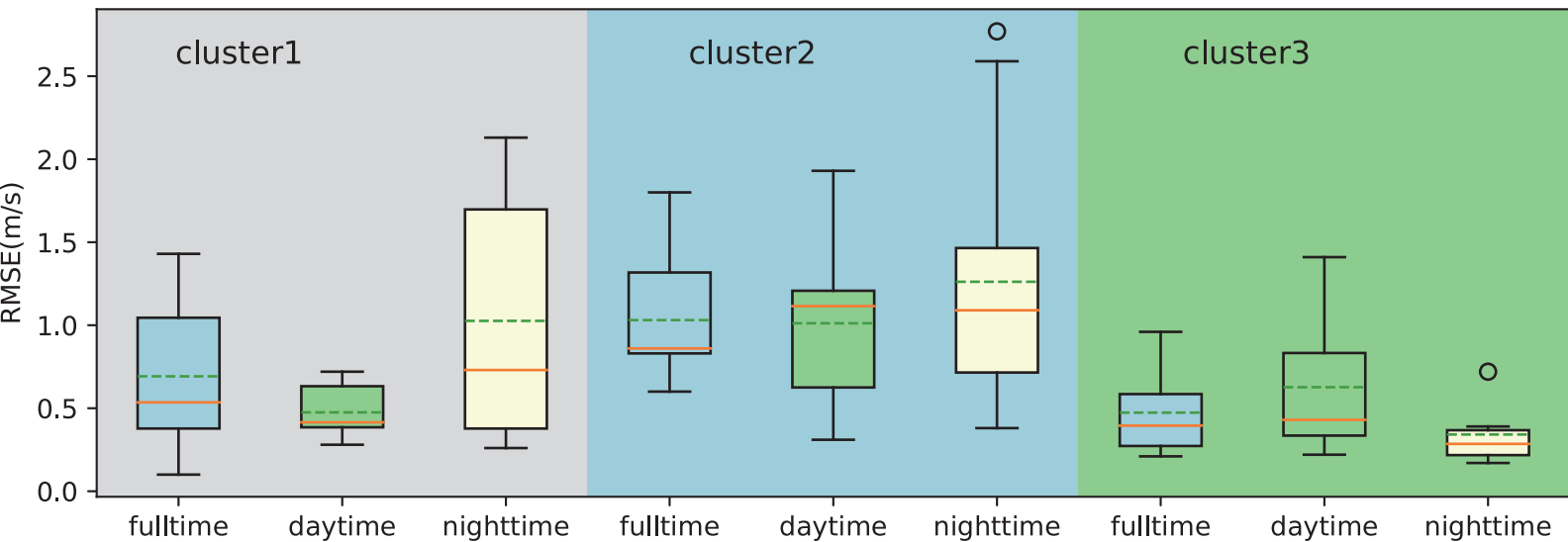
(a) RMSE Distribution in Different Clusters
