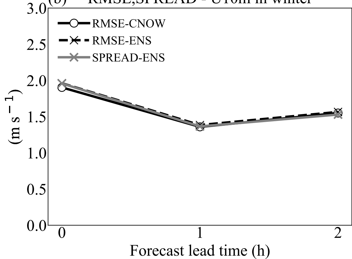
(b) RMSE, SPREAD - U10m in winter
