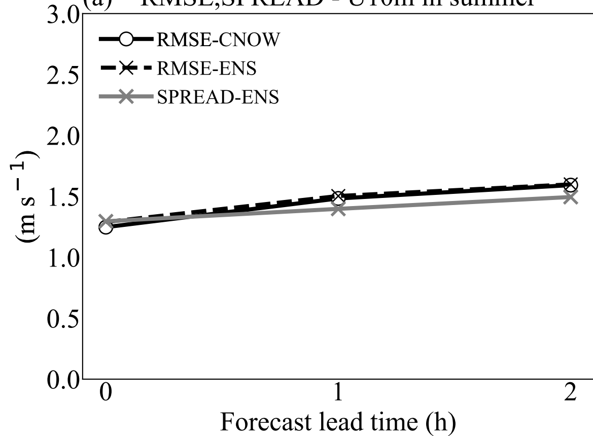
(a) RMSE, SPREAD - U10m in summer
