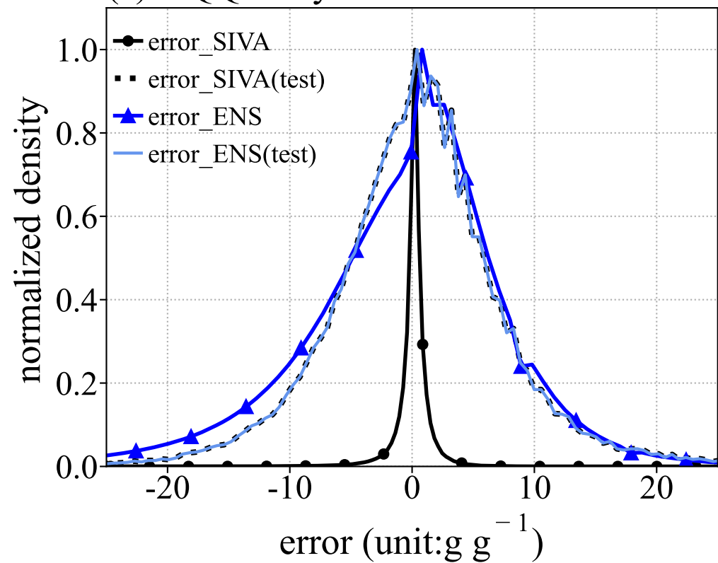
(c) QQ analysis errors in summer
