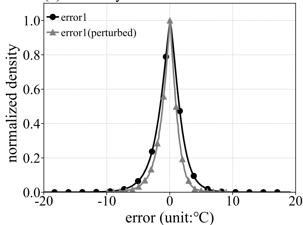
(c) QQ analysis errors in summer
