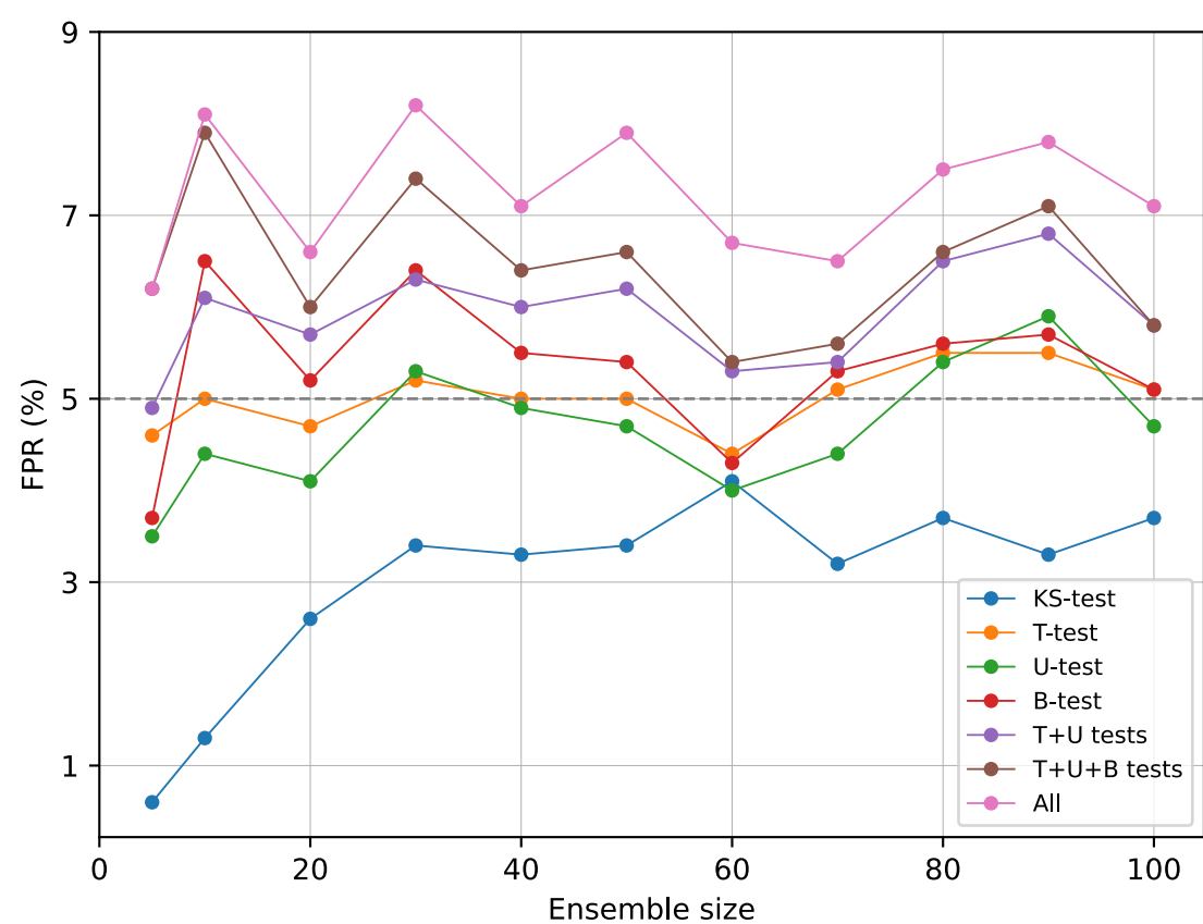
(a) FPR for Lorenz-96 ( F=8 ), RMSE
