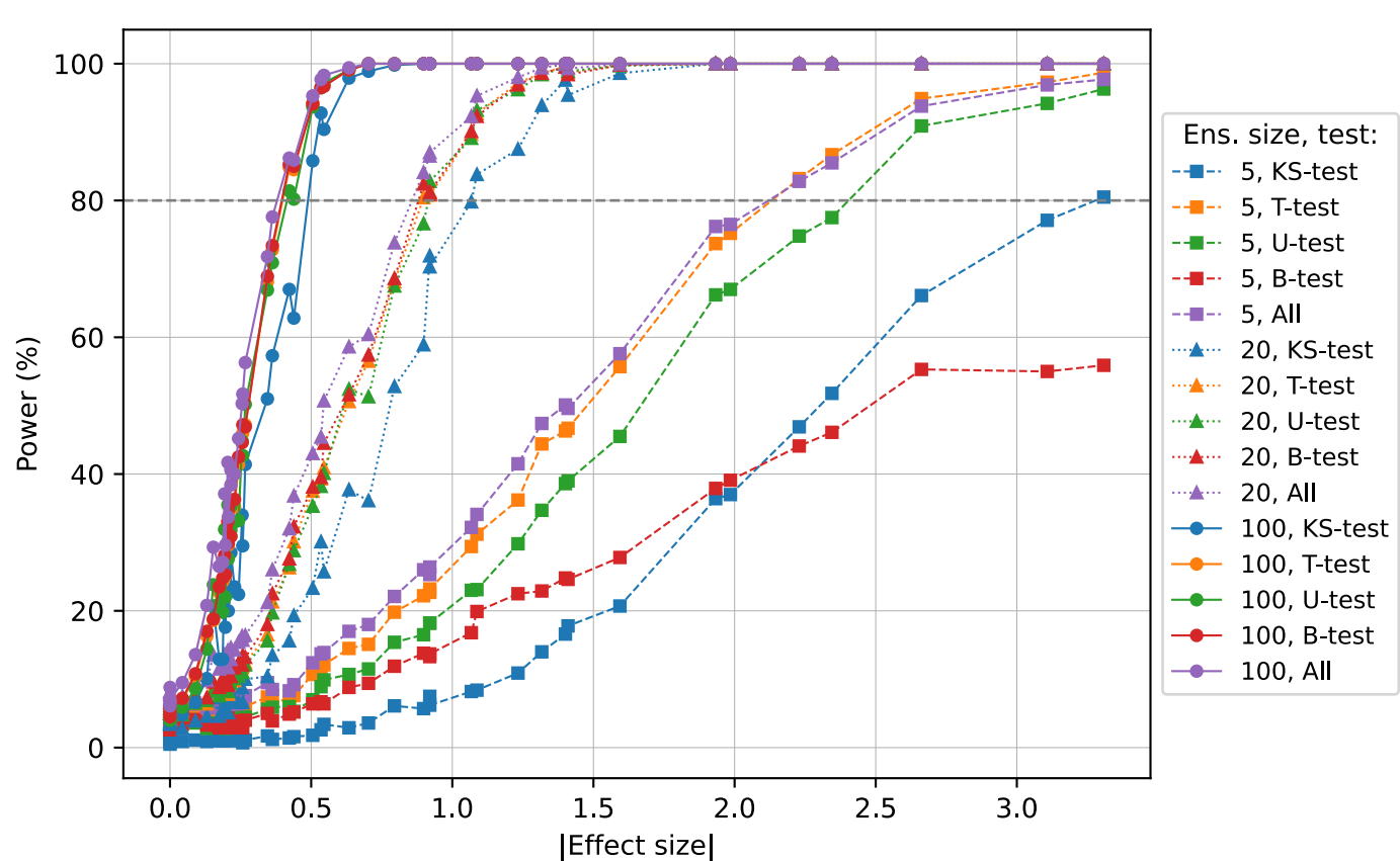
(b) Power for Lorenz-96 ( F_{ref}=8 )
