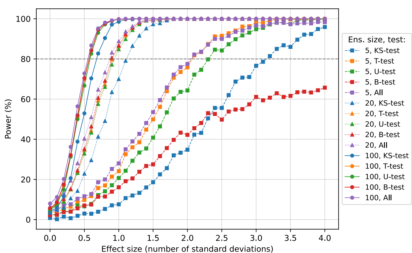
(b) Data from normal distributions ( \sigma=1 )
