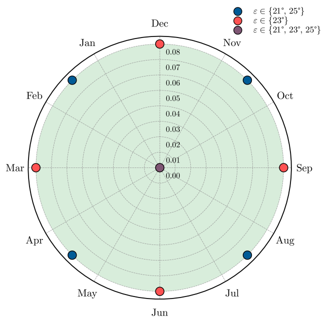
Figure 2. Slices of the cylinder constituting our HadCM3L experimental plan, with the eccentricity as the radius and the longitude of perihelion as the azimuthal angle. The angle is expressed in the month when the Earth is closest to the Sun, such that the vertical axis is the climatic precession e \sin \varpi and the horizontal axis is the coprecession e \cos \varpi . The colour is associated to obliquity \varepsilon being the third dimension. The green area illustrates the possible values used during the interpolation process.
