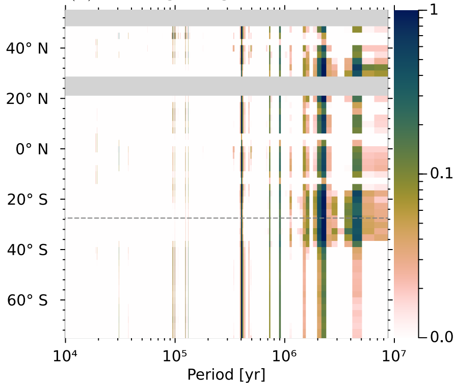
(a) Average regolith thickness
