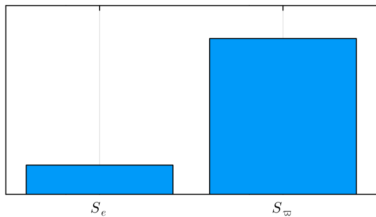
(f) \lambda_6/\lambda_{\text{tot}} = 0.0007
