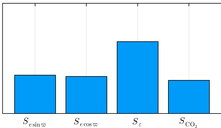
(e) \lambda_5/\lambda_{\text{tot}} = 0.0016
