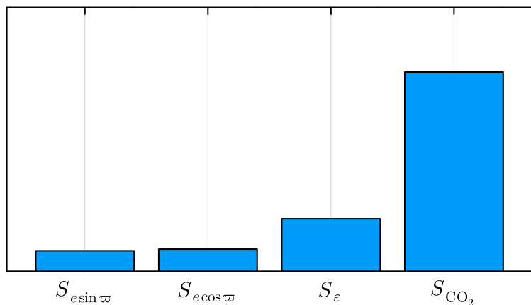
(f) \lambda_6/\lambda_{\text{tot}} = 0.0007
