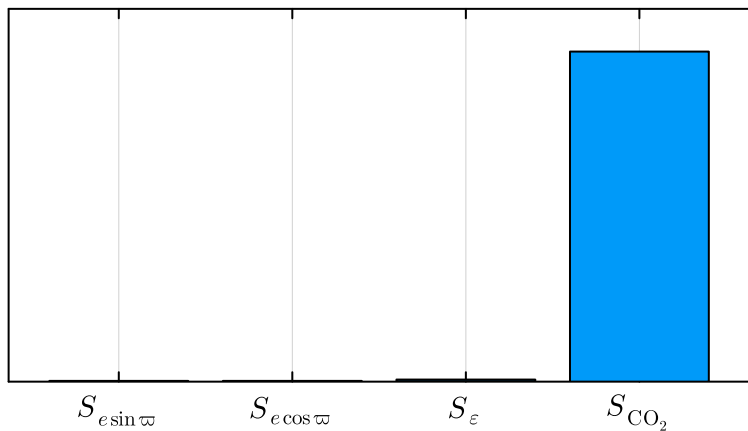
(c) \lambda_3/\lambda_{\text{tot}} = 0.0052
