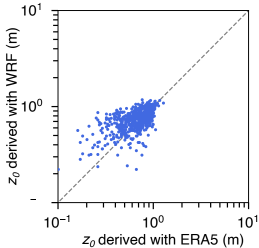
(a) z_0 derived from different sources
