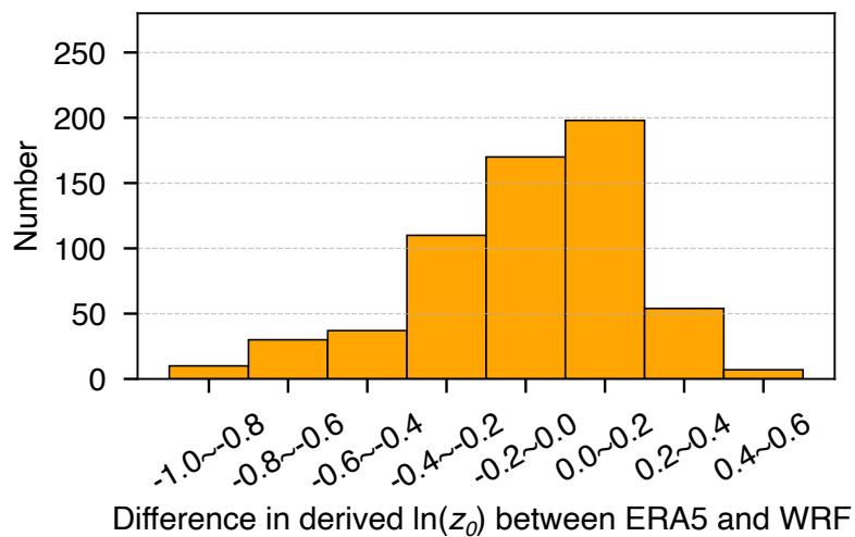
(c) Count of CMA stations across \ln(z_0) difference intervals
