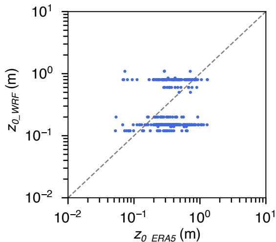
(a) Comparison of z_0 between WRF and ERA5
