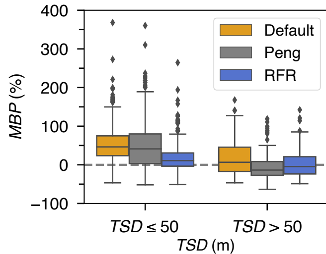
(c) MBP of 10-m wind speed for TSD categories
