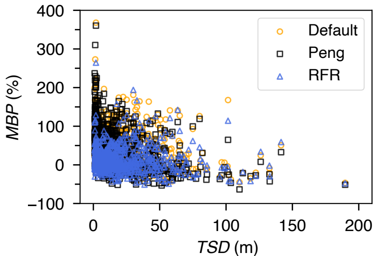
(b) MBP of 10-m wind speed distribution over TSD
