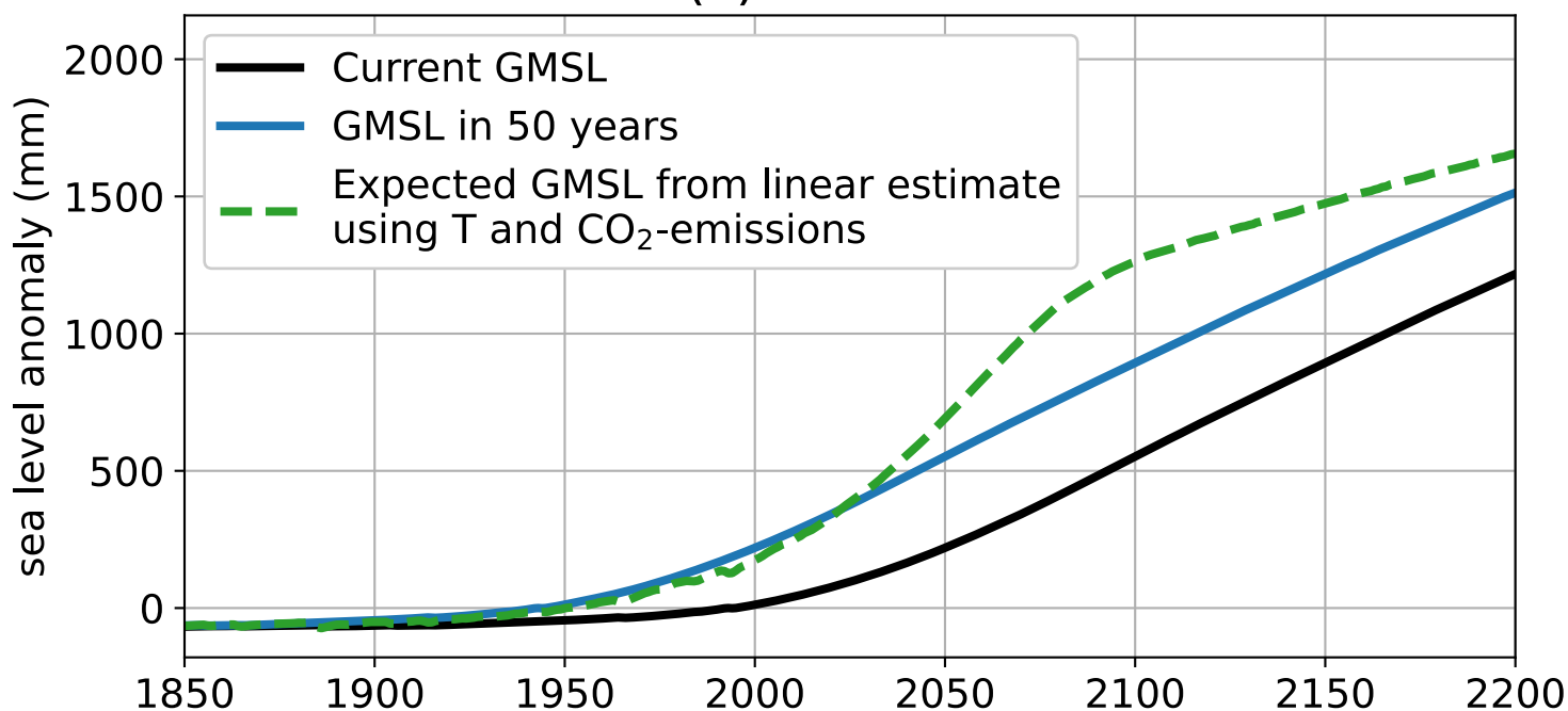
(c) SSP5-8.5
