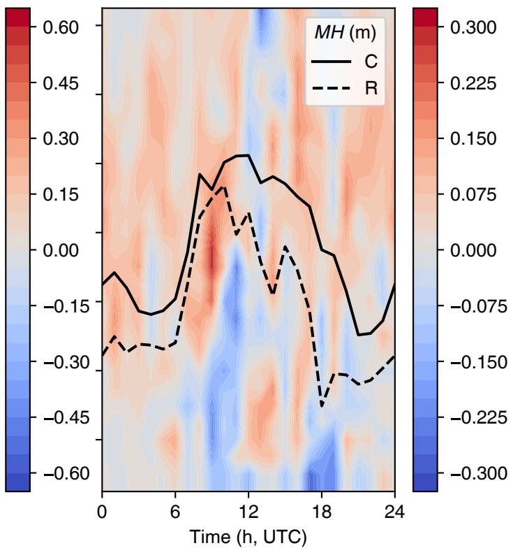
(c) \Delta q ( \text{g kg}^{-1} )
