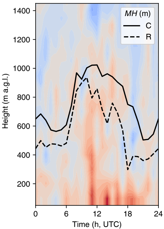
(b) \Delta\theta (K)
