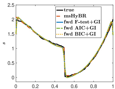
(c) Forward selection methods.
