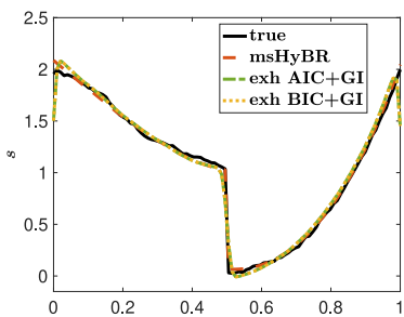
(b) Exhaustive selection methods.
