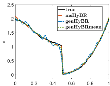
(a) Bayesian approaches.
