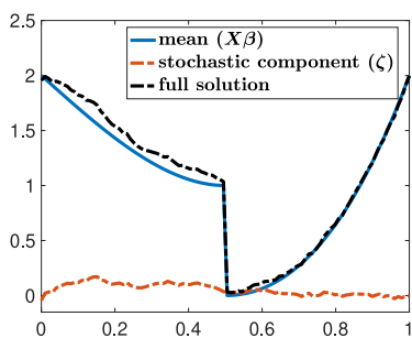
(c) True solution.
