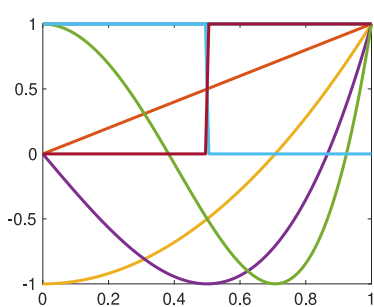
(a) Basis vectors.
