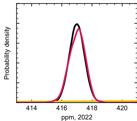
CO 2 concentration
