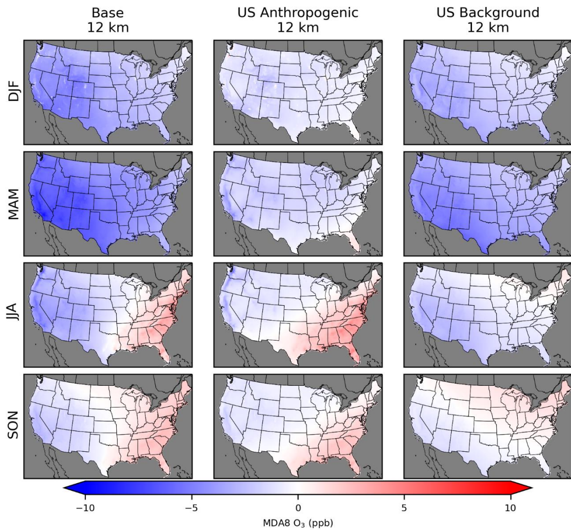
Figure S11. Seasonal average of inferred MDA8 O 3 model bias from 12 km horizontal resolution EQUATES CMAQ simulations. O 3 concentrations include total (base) O 3 as well as O 3 components from US anthropogenic and US background sources.
