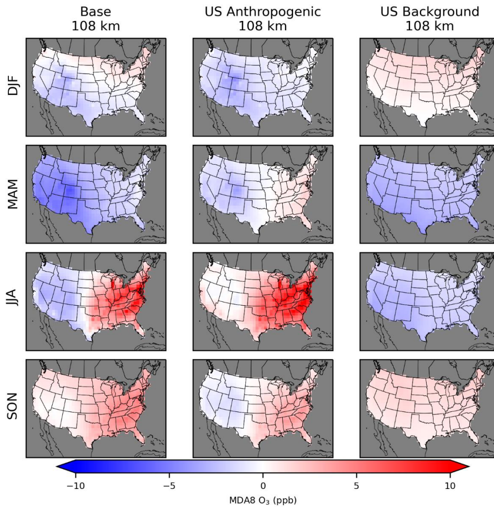
Figure S12. Seasonal average of inferred MDA8 O 3 model bias from 108 km horizontal resolution EQUATES CMAQ simulations. O 3 concentrations include total (base) O 3 as well as O 3 components from US anthropogenic and US background sources.
