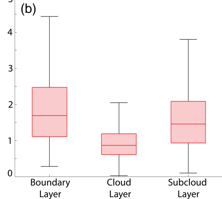
Zonal Shear from ERA5 trajectories [ \text{m/s} ]
