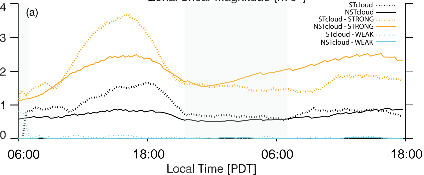
Zonal Shear Magnitude [ \text{m s}^{-1} ]
