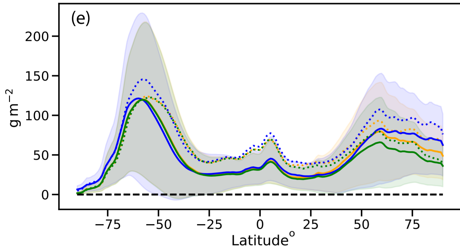
ACTNL Ensemble Mean and SD
