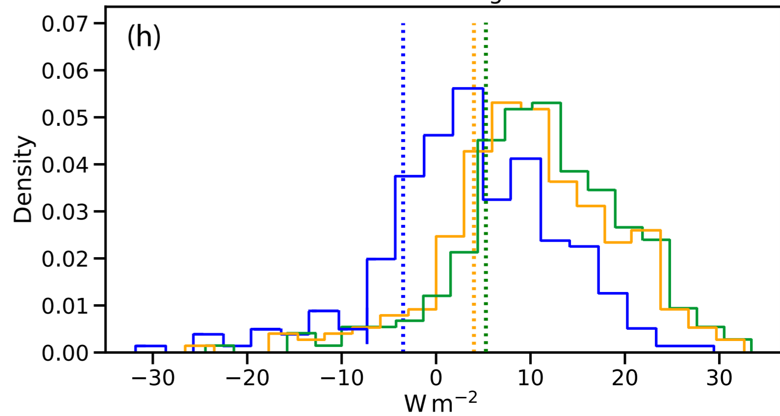
TOA Histogram
