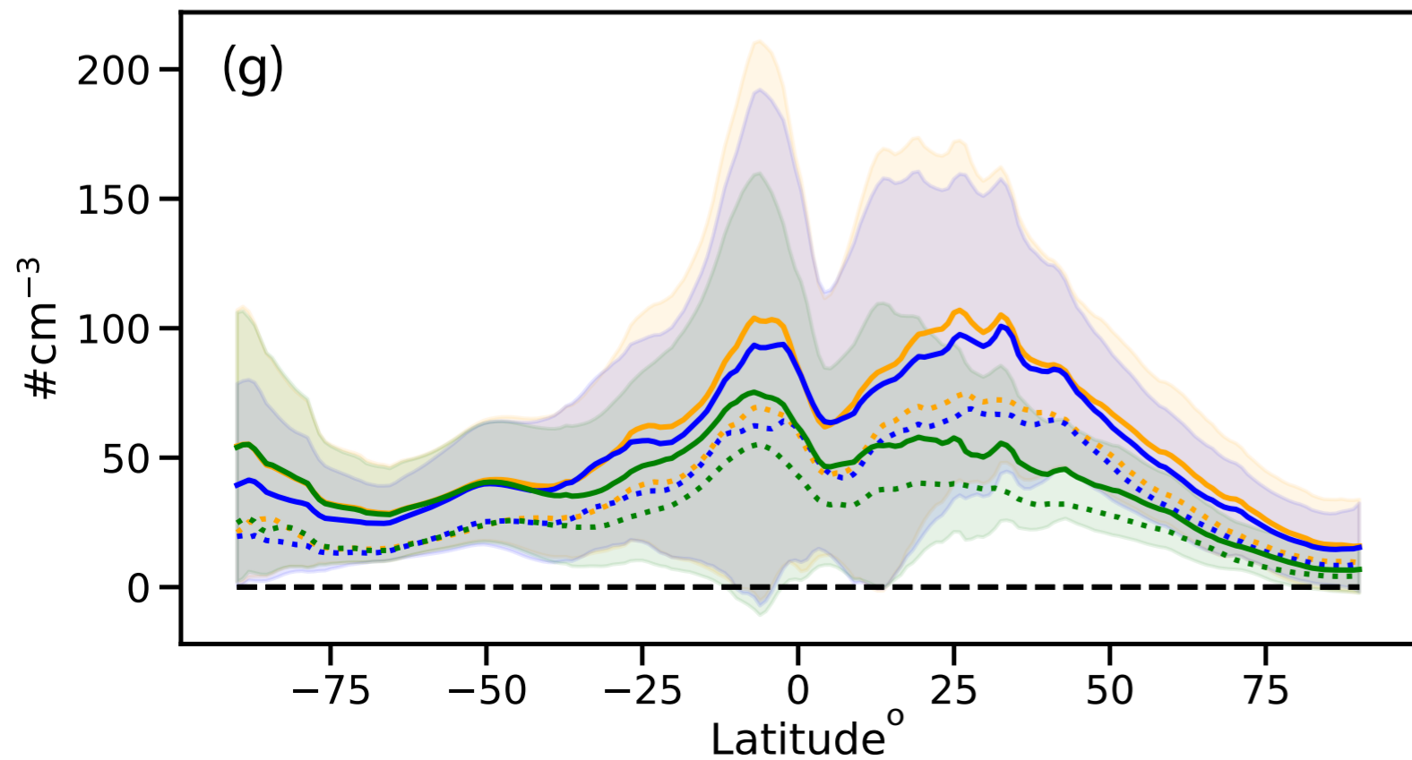
ACTNL Ensemble Mean and SD
