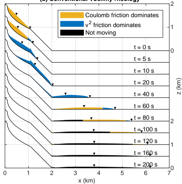
(b) Conventional Voellmy rheology
