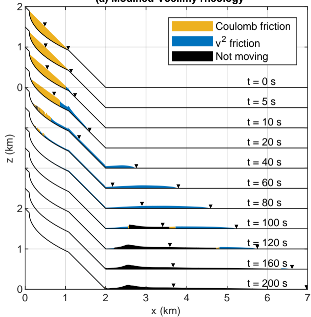
(a) Modified Voellmy rheology
