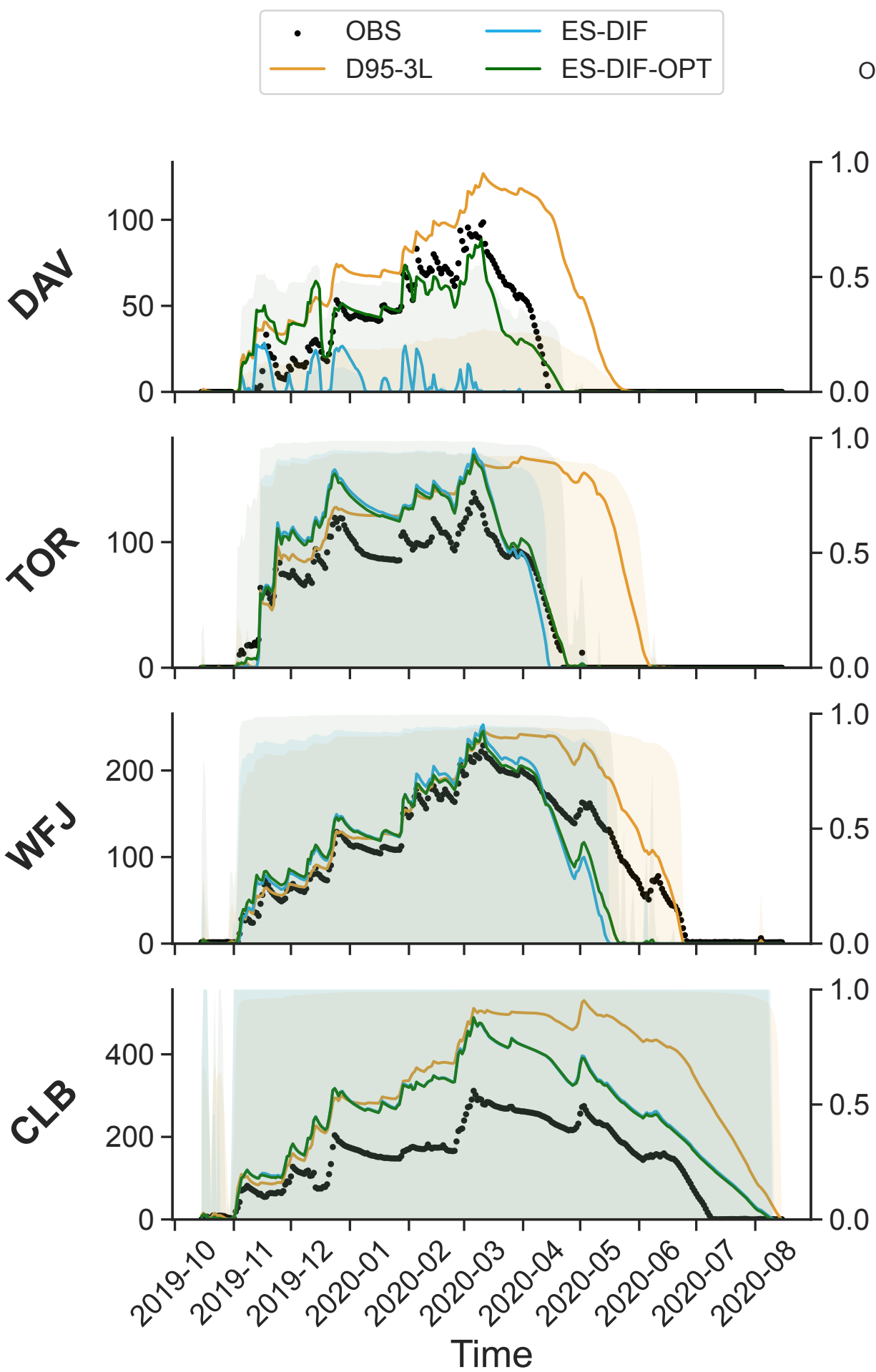
(a) Time series of snow depth (cm) and snow cover fraction
