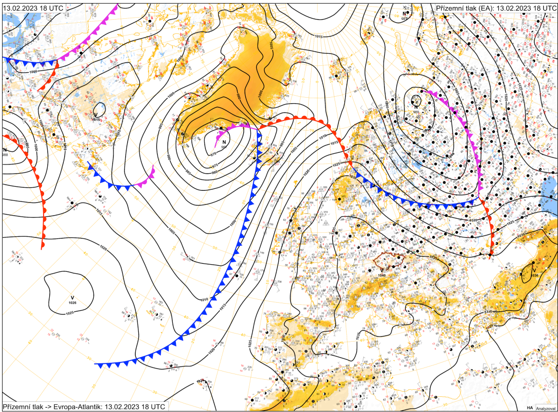
Figure S4: Surface pressure map and cloud cover over the Atlantic and Europe for 13 February 2023, 18 UTC. Map provided by CHMI.
