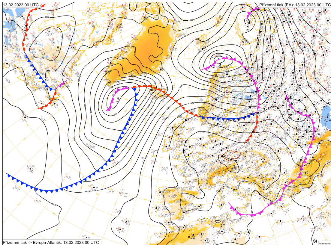
Figure S1: Surface pressure map and cloud cover over the Atlantic and Europe for 13 February 2023, 00 UTC. Map provided by Czech Hydrometeorological Institute (CHMI).
