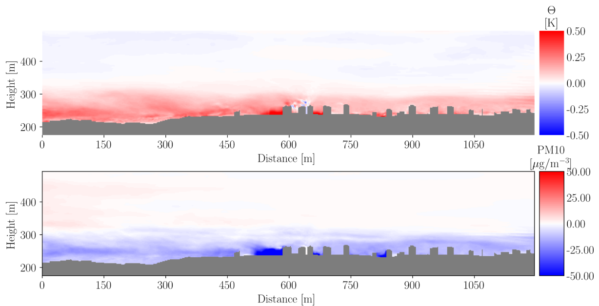
Fig. 21: Difference of HEAT minus BASE scenarios for PALM-ICON model on 13 February 2023 at hour 18. The values of air temperature (upper) and concentration of PM 10 (lower) on the cross-section through the child domain in the position of ALEGA station are shown.
