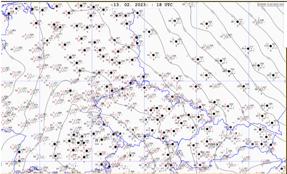
Figure S8: Surface weather analysis with isobars (black) for 13.2. 18:00 UTC. Map provided by CHMI.
