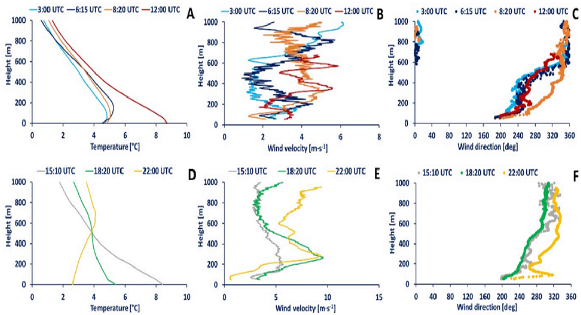
Figure S9: Temperature (A+D), wind velocity (B+E) and wind direction (C+F) profiles measured during 13 February 2023 in Prague TURBAN observation campaign. Change in temperature stratification within the lower boundary layer at selected morning and afternoon hours.
