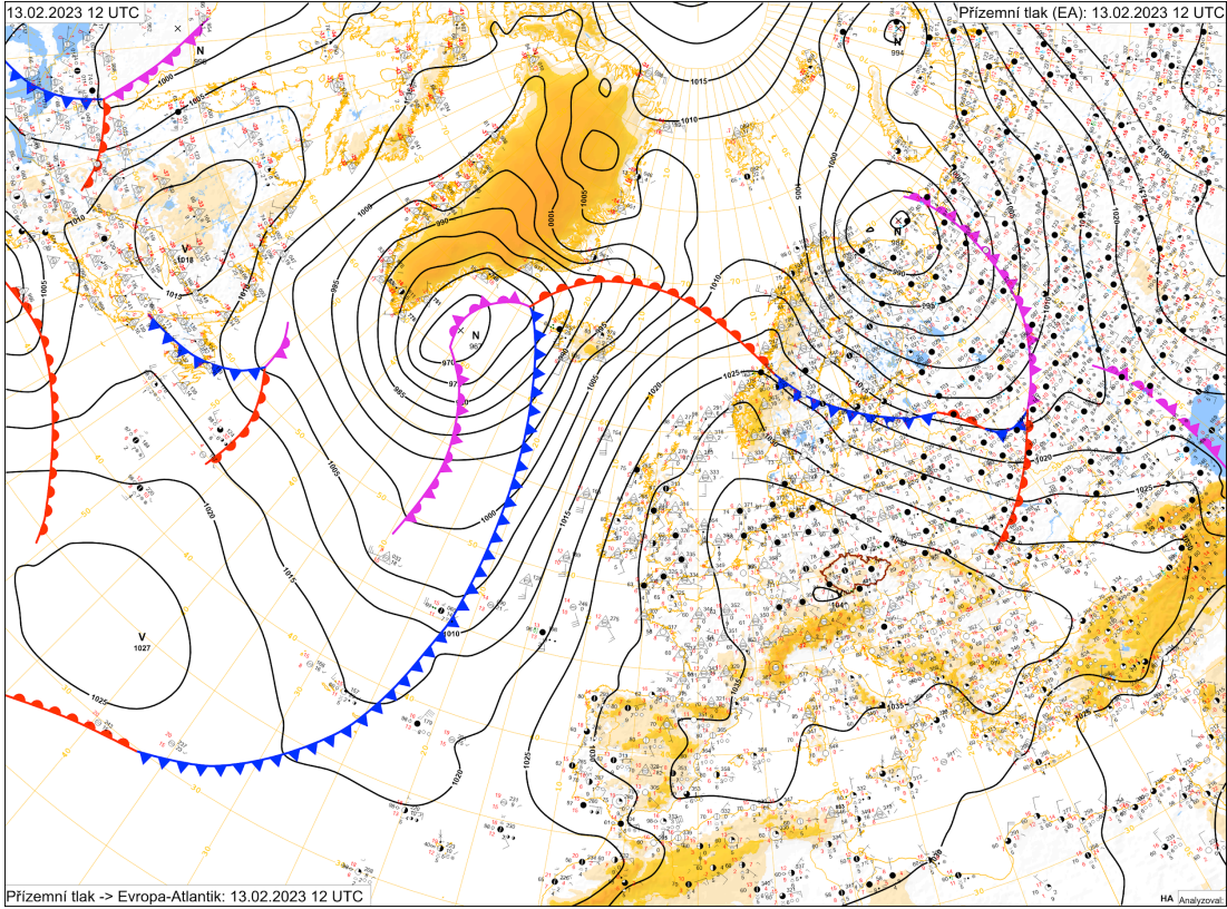
Figure S3: Surface pressure map and cloud cover over the Atlantic and Europe for 13 February 2023, 12 UTC. Map provided by CHMI.
