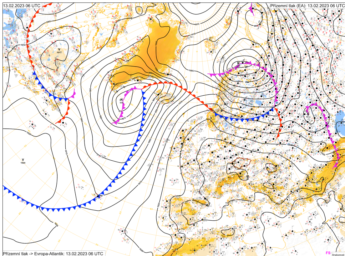
Figure S2: Surface pressure map and cloud cover over the Atlantic and Europe for 13 February 2023, 06 UTC. Map provided by CHMI.
