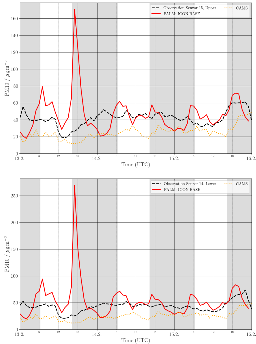
Fig. S15: Comparison of the PALM modeled and observed concentrations of PM_{10} on the sensors S14 and S15. Observations are represented by the black dashed line and the ICON base scenario is shown by the solid red line. The orange dotted line (CAMS) represents the analysis of the observations and CAMS model used as the BC.
