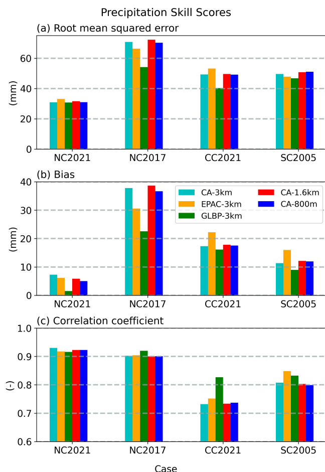
Figure 6. Skill scores for the event accumulated precipitation for each case and grid configuration as computed with respect to PRISM observations. Displayed are the (a) root mean squared error, (b) bias, and (c) Pearson pattern correlation coefficient.
