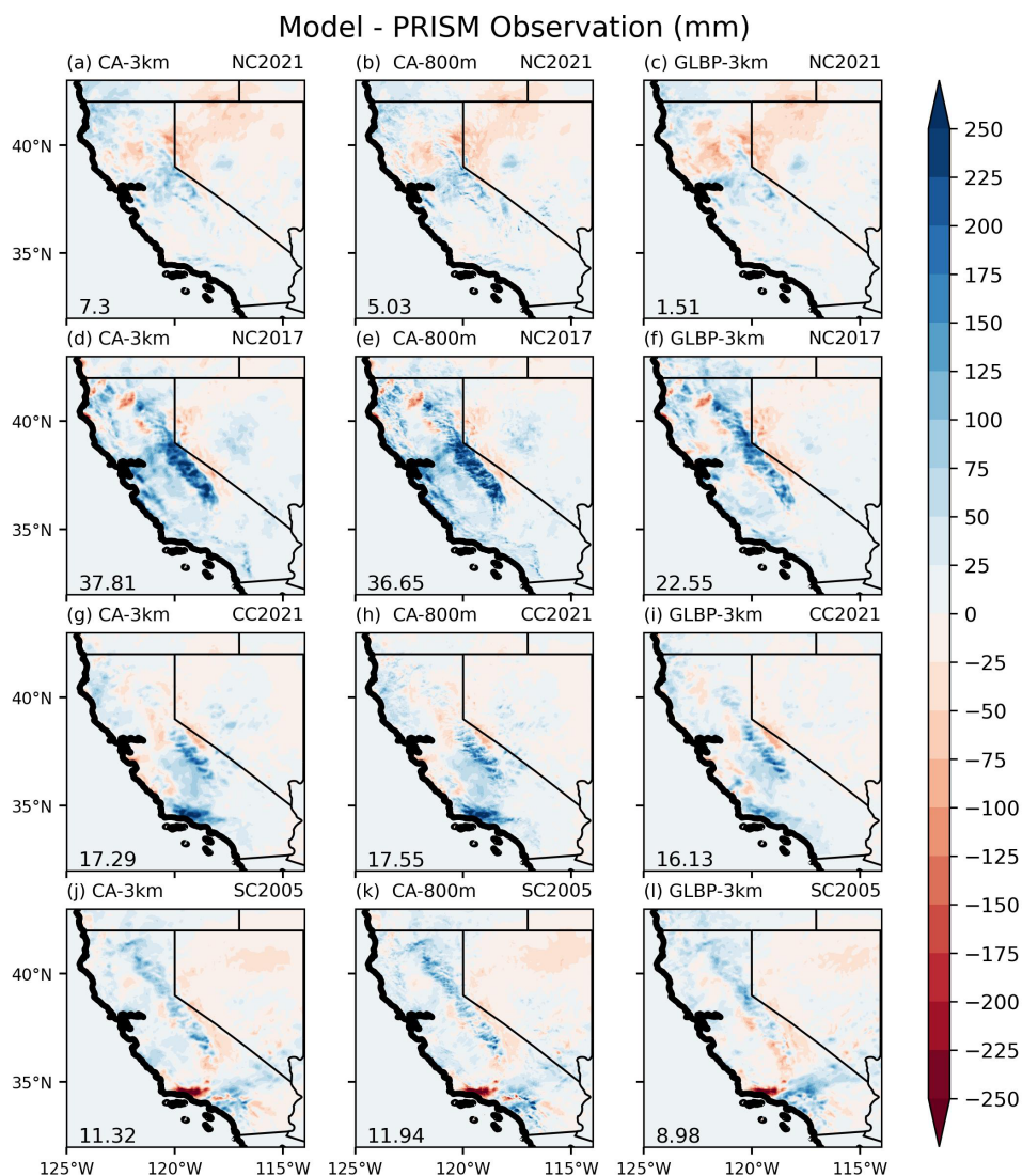
Figure 8. Event accumulated precipitation bias computed relative to PRISM observations for (left column) CA-3km RRM, (middle column) CA-800m, and (right column) GLBP-3km for each case. The numerical value in the bottom left corner of each panel represents the averaged bias over CA. Model simulations are remapped to PRISM resolution to compute bias.
