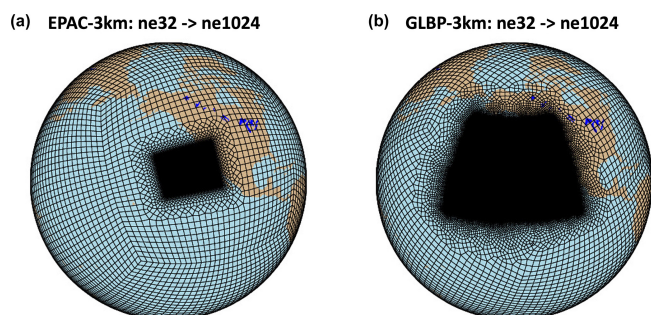
Figure 2. Depiction of the grid mesh used for the (a) EPAC-3km and (b) GLBP-3km grid configurations. Both configurations have ne1024 ( \sim 3 km) resolution within the refined region and ne32 ( \sim 100 km) resolution outside this region.
