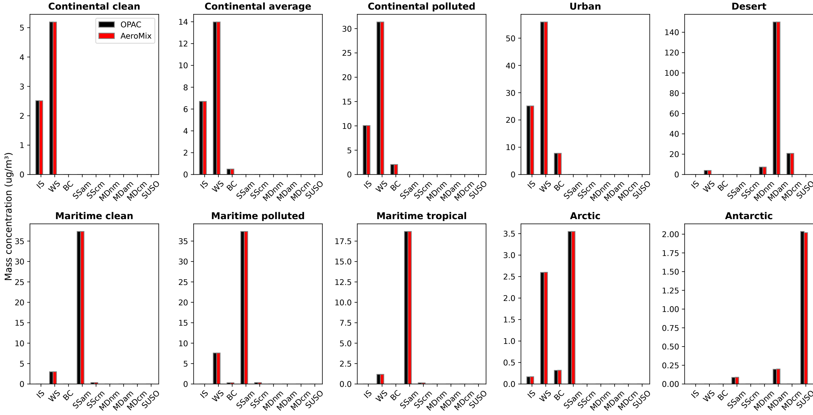
Aerosol components
