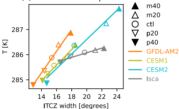
(a) Global mean temperature
