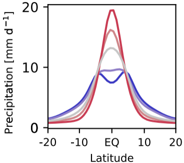
(a) Zonal mean climatology
