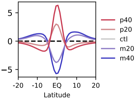
(b) Difference from itcz-slab
